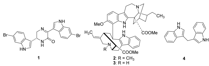
Figure 1. Structures of biologically active bisindole alkaloids 1-4
