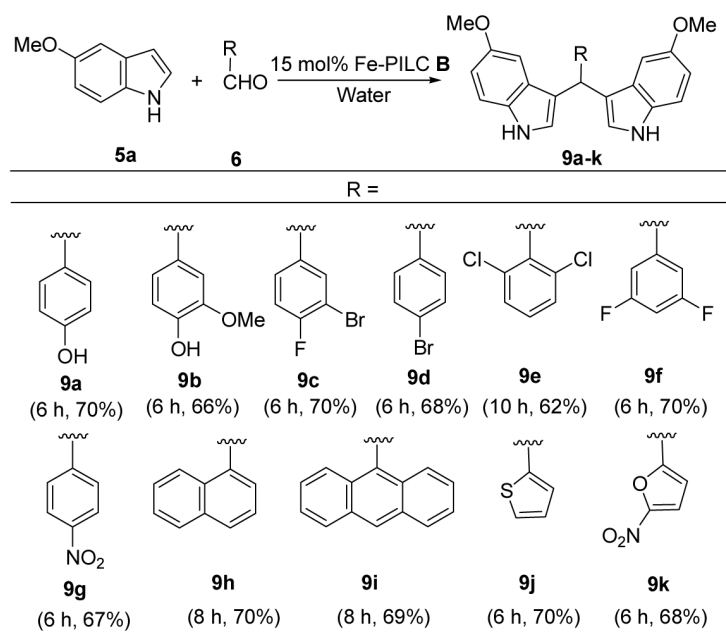
Figure 5. Synthesis of 5,5'-dimethoxy-3,3'-diindolylmethanes 9a-k
