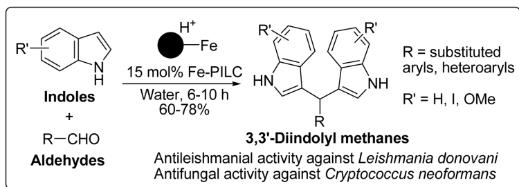
Figure 2. Synthesis of 3,3'-diindolylmethanes using Fe-PILC catalyst
