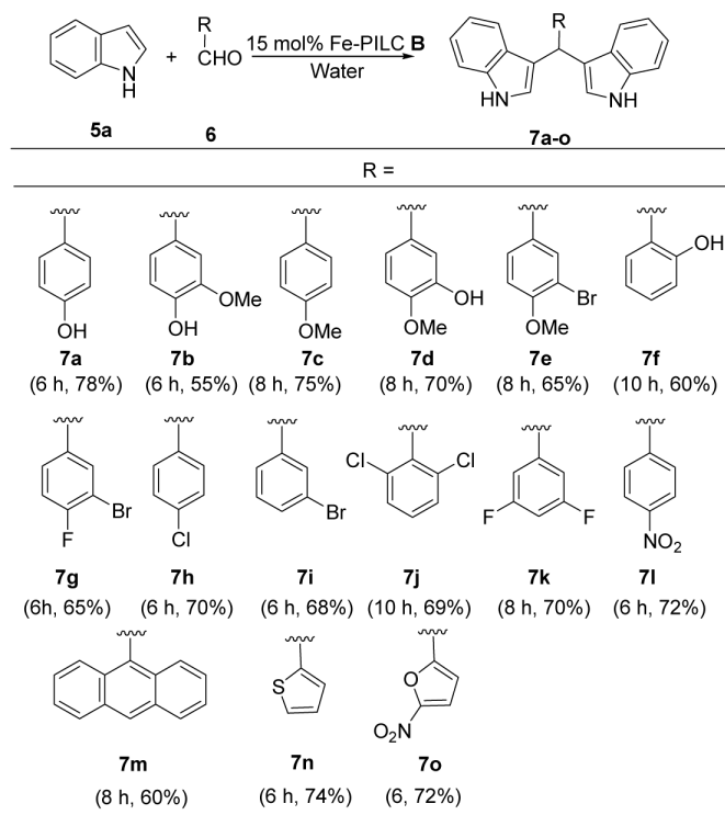
Figure 3. Synthesis of 3,3'-diindolylmethanes 7a-o
