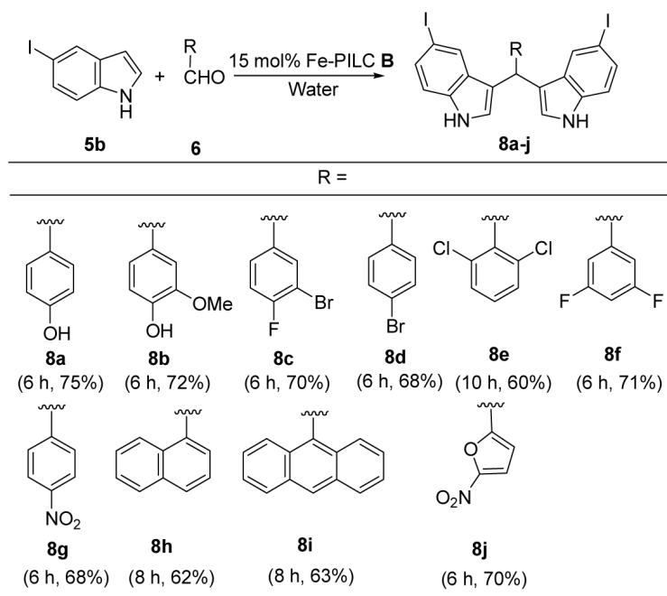
Figure 4. Synthesis of 5,5'-diiodo-3,3'-diindolylmethanes 8a-j
