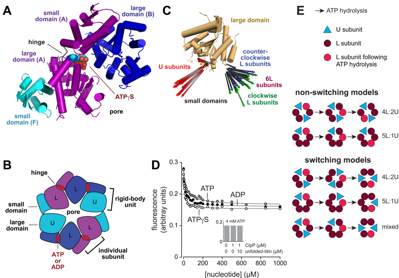
Figure 1. ClpX structure
