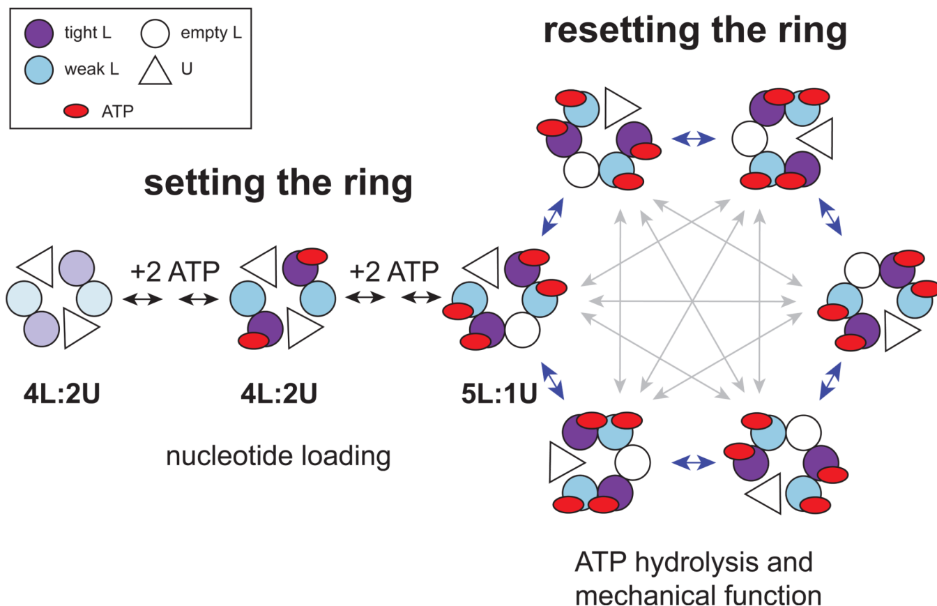
Figure 7. Model for ring-setting and ring-resetting reactions
