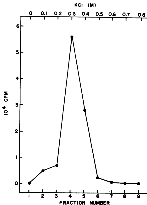
FIG. 1. Phosphocellulose column chromatography of an enzyme extract prepared from PBCV-1-infected Chlorella cells at 3 h post-infection. Protein (33 mg) was applied to the column and eluted stepwise with 0 to 0.8 M KCl. Fractions (1 ml) were collected, and 10 \mu l of the middle fraction at each salt concentration was assayed for DNA methyltransferase activity with 3 \mu g of unmethylated lambda DNA as a substrate.
