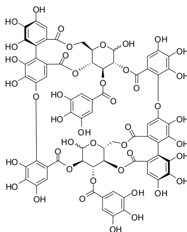
Figure 1. Structure of oenothin B.
