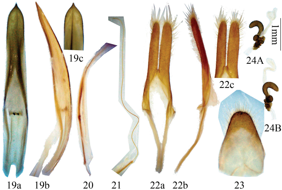
Figures 19–24. Genitalia of Distenia japonica Bates, 1873. 19–23 male, from Kyoto, Japan 19 median lobe 20 rods of endophallus 21 hair-like thin rod of ejaculatory duct 22 tegmen. a ventral view b lateral view c dorsal view 23 tergite VIII in dorsal view 24 female, spermathecal capsule, from Kyoto, Japan. A–B from different sides. Scale 1 mm.
