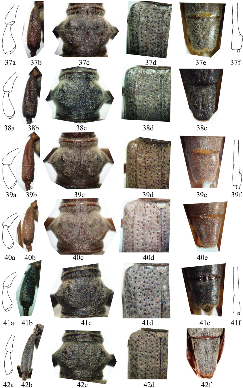
Figures 37–42. Six important characters of Distenia spp. not to scale. 37–38 D. gracilis . 37 male from Far East, Russia 38 female from Liaoning, China 39–40 D. japonica 39 male from Kyoto, Japan 40 female from Kyoto, Japan 41–42 D. orientalis sp. n. 41 male from Tianmushan, China 42 female from Tianmushan, China a last segment of maxillary palp, showing the tip and the ration of length to width b scape c pronotum d basal part of elytron e ventrite V f mesotibia of male, showing the apical protruding lobe.
