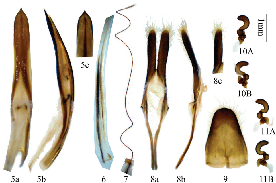
Figures 5–11. Genitalia of Distenia gracilis (Blessig, 1872). 5–9 male, from Far East Russia 5 median lobe 6 rods of endophallus 7 hair-like thin rod of ejaculatory duct 8 tegmen a ventral view b lateral view. c dorsal view 9 tergite VIII in dorsal view 10–11 female, spermathecal capsule, both from Liaoning, China. A–B from different sides. Scale 1 mm.
