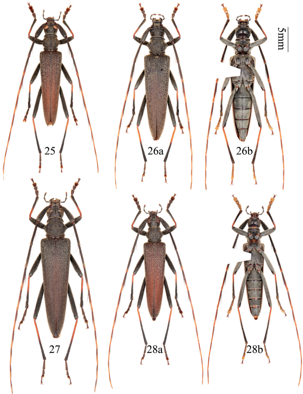
Figures 25–28. Distenia orientalis sp. n. 25 holotype, male, from Xitianmushan, Zhejiang, China 26 paratype, female, from Tianmushan, Zhejiang, China 27 paratype, female, from Fengyangshan, Zhejiang, China 28 paratype, male, from Wuyishan, Fujian, China a dorsal view b ventral view. Scale 5 mm.
