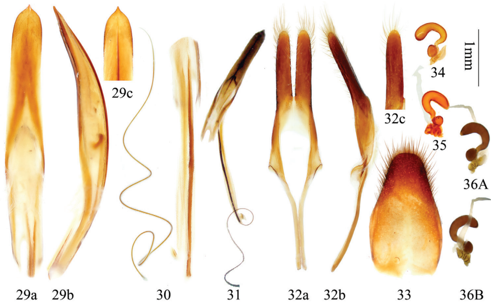
Figures 29–36. Genitalia of Distenia orientalis sp. n. 29–33 male, from Xitianmushan, Zhejiang, China 29 median lobe 30 rods of endophallus and hair-like thin rod of ejaculatory duct 31 whole median lobe, showing the position of rods of endophallus, not to scale 32 tegmen a ventral view b lateral view c dorsal view 33 tergite VIII in dorsal view 34–36 female, spermathecal capsule 35 from Fengyangshan, Zhejiang, China 34 & 36 from Tianmushan, Zhejiang, China. A & B from different sides. Scale 1 mm.
