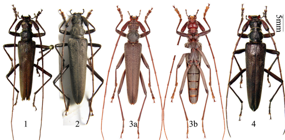
Figures 1–4. Distenia gracilis (Blessig, 1872). 1 male, from Far East Russia 2 female, from Far East Russia 3 male, from Liaoning, China a dorsal view b ventral view 4 female, from Liaoning, China. Scale 5 mm.
