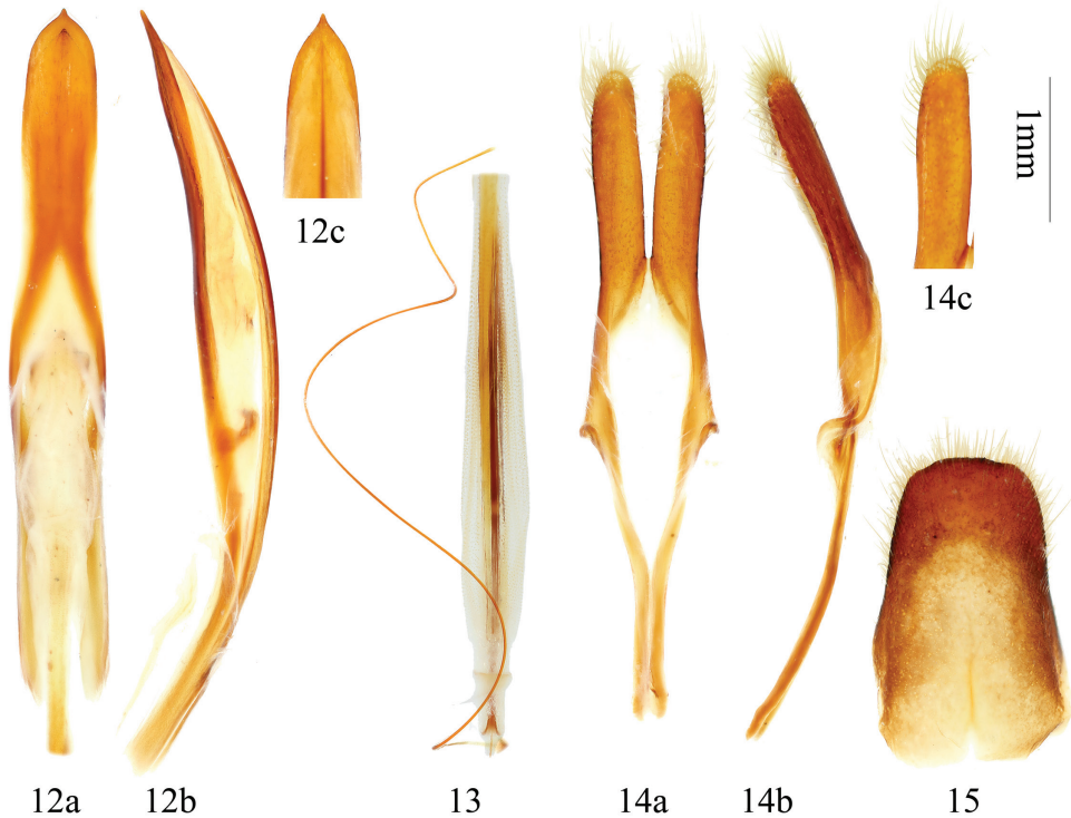
Figures 12–15. Genitalia of Distenia gracilis (Blessig, 1872), male, from Liaoning, China 12 median lobe 13 rods of endophallus, including hair-like thin rod of ejaculatory duct 14 tegmen a ventral view b lateral view c dorsal view 15 tergite VIII in dorsal view. Scale 1 mm.
