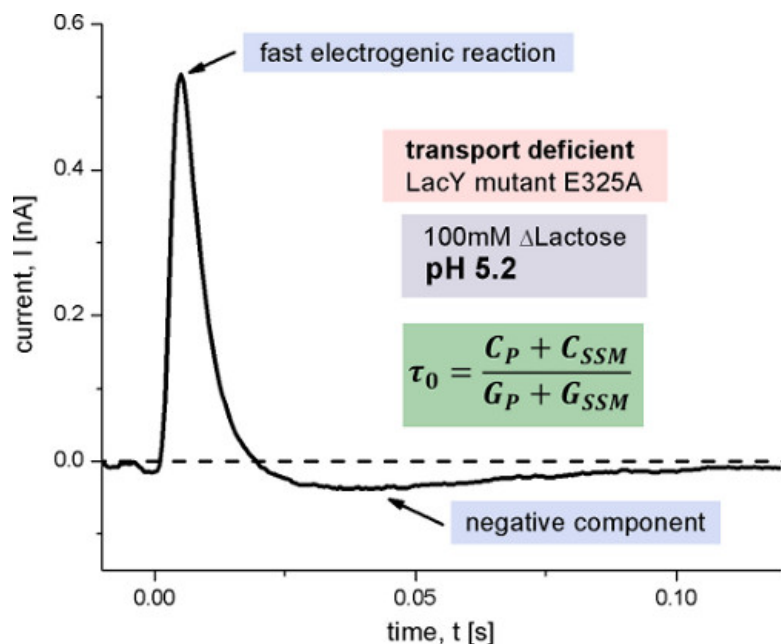
Figure 7. Transient current measured with E325A LacY proteoliposomes after a 100 mM lactose concentration jump at pH 5.2. This LacY variant is inhibited in the proton release step of the transport cycle and therefore transport-deficient. The small negative component observed is characteristic for rapid transient currents measured in capacitively coupled systems and is caused by the discharge of the membrane capacitance after a fast electrogenic reaction. Its time constant \tau_0 is determined by the capacitances and conductances of the system (Figure 1).
