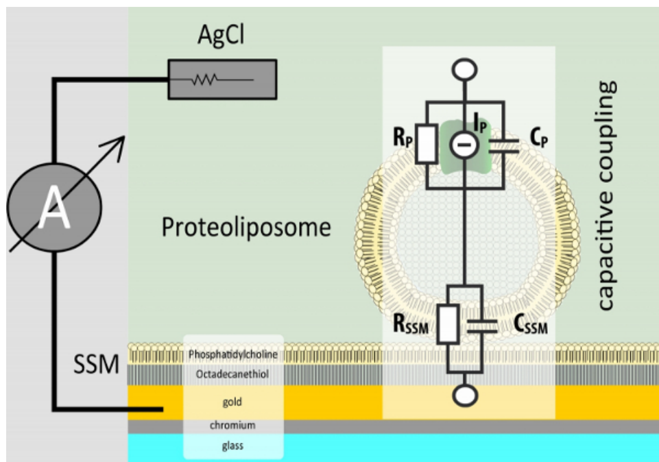
Figure 1. Adsorption geometry of proteoliposomes on the SSM. The SSM is formed on a sensor chip, a structured gold coated glass slide. To measure electrogenic reactions of membrane proteins, proteoliposomes or membrane fragments are adsorbed to the SSM. The two membranes form a capacitively coupled system. This is why only transient currents are detected.
