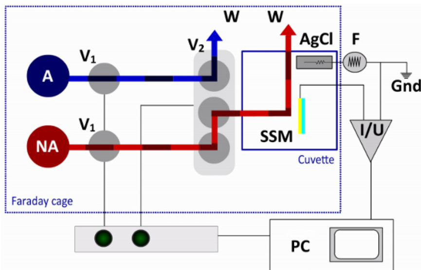
Figure 3. Fluid Pathway and Electrical Circuit of the SSM Setup. In the single solution exchange protocol only one non-activating (NA) and one activating (A) solution are required. The flow is controlled by two 2-way valves (V1) and one terminal valve (V2). The terminal valve switches between non-activating and activating solutions, directing one of the solutions to the cuvette and the other solution to a waste container (W). The sensor chip (SSM) is connected to the amplifier (I/U), while the reference electrode (AgCl) is connected to the function generator (F) in the external electrical circuit. A computer (PC) and an interface box are used for valve operation and data acquisition.
