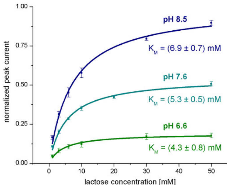
Figure 5. Averaged normalized Peak currents measured with wild-type LacY proteoliposomes after lactose concentration jumps at different concentrations and pH values. The K_M values are obtained from the hyperbolic fits.
