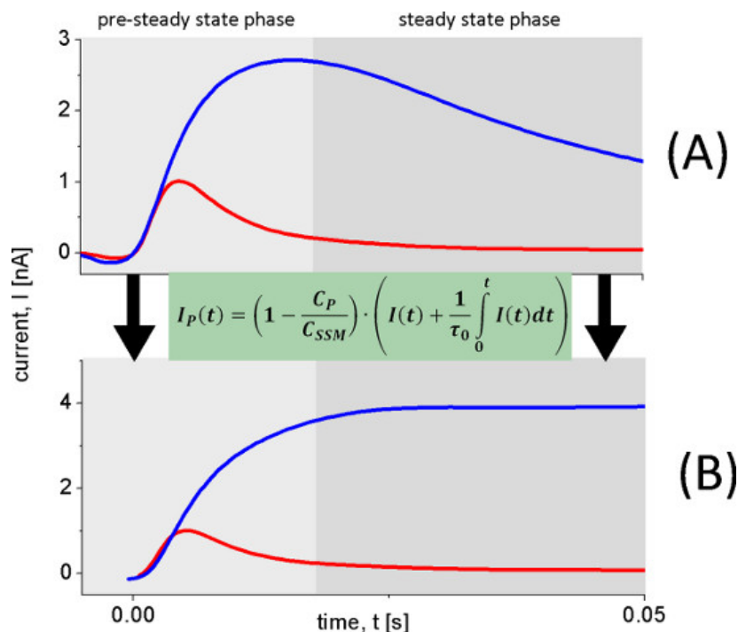
Figure 6. Reconstruction of transporter currents. The transient currents (A) used to reconstruct the transporter currents (B) were measured with wild-type LacY proteoliposomes after 100 mM lactose concentration jumps at pH 8.5 (blue trace) and pH 5.2 (red trace). At pH 8.5 continuous turnover is observed while at pH 5.2 a fast electrogenic reaction occurs. This is clearly observed in the reconstructed current (B).
