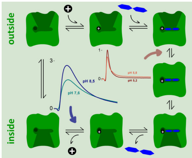
Figure 9. A kinetic model for the reaction cycle of LacY. Two electrogenic steps could be identified and characterized by SSM measurements. A strongly electrogenic reaction representing ~94% of the total charge displacement in the reaction cycle is only observed at neutral and basic pH values. It could be assigned to the proton release step (blue arrow). A weakly electrogenic step is observed at acidic pH when continuous turnover of wild-type LacY is inhibited. We assigned this reaction to an electrogenic conformational transition upon lactose binding, which represents 6% of the total charge displacement in the reaction cycle.
