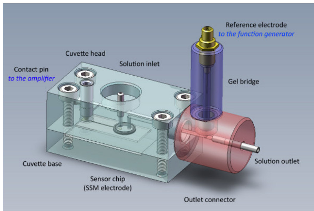
Figure 2. The SSM cuvette carries the sensor chip and the reference electrode. The sensor chip is sandwiched between the cuvette base and the cuvette head. The reference electrode is isolated from the flow pathway by a polyacrylamide gel salt bridge.
