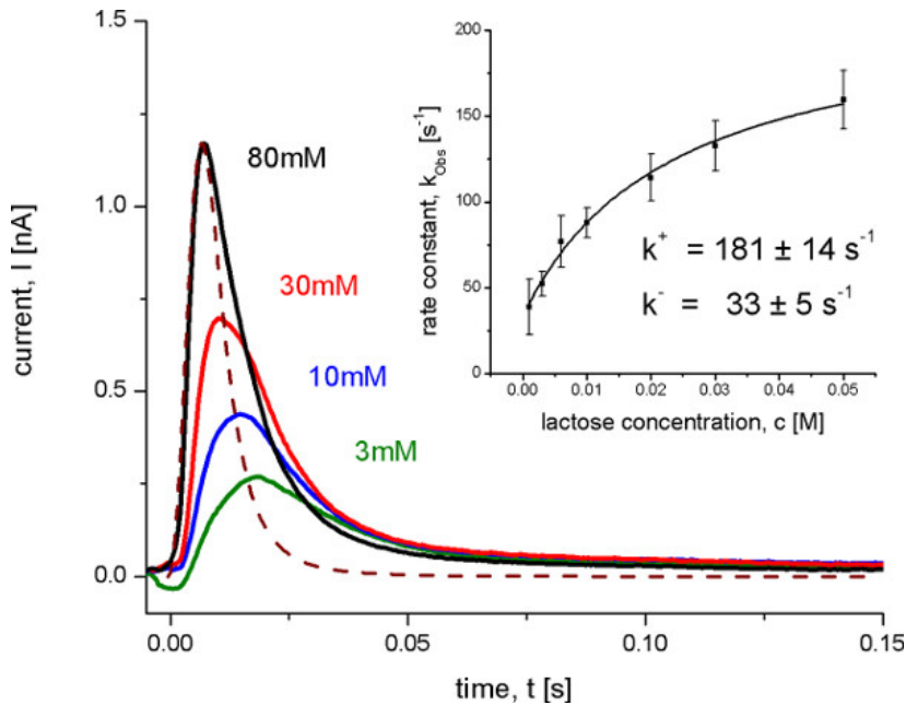
Figure 8. Transient currents measured with wild-type LacY proteoliposomes after different lactose concentration jumps at pH 5.2. Under these conditions no steady state transport is observed, but an electrogenic conformational transition upon lactose binding. The dashed line shows the transfer function representing the time resolution of the system. The inset shows the determination of the on and off rate constants from the observed rate constant k_{obs} with a hyperbolic fit to the data. The observed rate constant was determined from the transient currents with an iterative least-squares deconvolution algorithm 10 .
