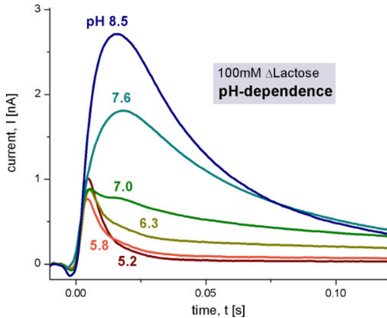
Figure 4. Transient currents measured with wild-type LacY proteoliposomes after 100 mM lactose concentration jumps at different pH values. The non-activating solution contained 100 mM glucose while the activating solution contained 100 mM lactose. All solutions were prepared in 100 mM potassium phosphate buffer at the indicated pH with 1 mM DTT. For details of measurement conditions in this and the following figures please refer to 9 and 10 .
