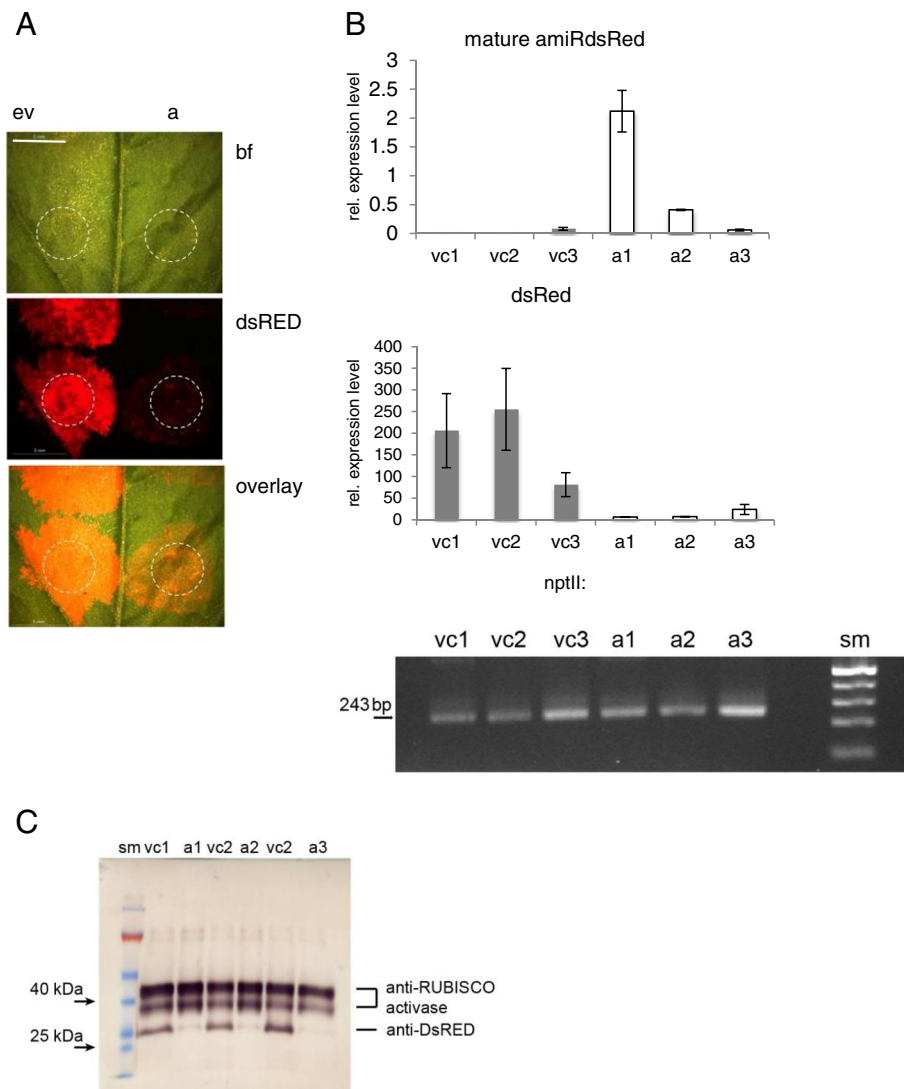
Figure 2 The mt-miR159b-mediated amiR-silencing is efficient in tobacco leaves. A) DsRED fluorescence is strongly reduced after infiltration of the pRed-35Spro::amiR-dsred ( A ) construct (a) as compared to empty vectors (ev). Bright field image (bf), DsRED fluorescence (dsRED) and an overlay of both channels are shown. Infiltration site are indicated by dotted lines. Scale bar: 5 mm. B) Relative levels of mature amiR-dsred determined by stem loop qRT-PCR, relative transcript levels of dsred measured by qRT-PCR and transcript levels of nptII (kanamycin resistance) are shown. vc: vector controls, a: amiR samples sm: size marker, amplicon size of 243 bp is indicated. C) Western blot demonstrating reduced expression of dsRED after amiR-dsred mediated silencing of dsRED in tobacco leaves. Shown are three replicates of amiR-silencing (a) and vector controls (vc) represented by proteins of three different infiltration spots on the same leaf, for each construct. Reduced expression of dsRED after amiR-dsred infiltration was visualized using an anti-dsRED antibody. Equal sample loading is shown by anti-RUBISCO activase.
