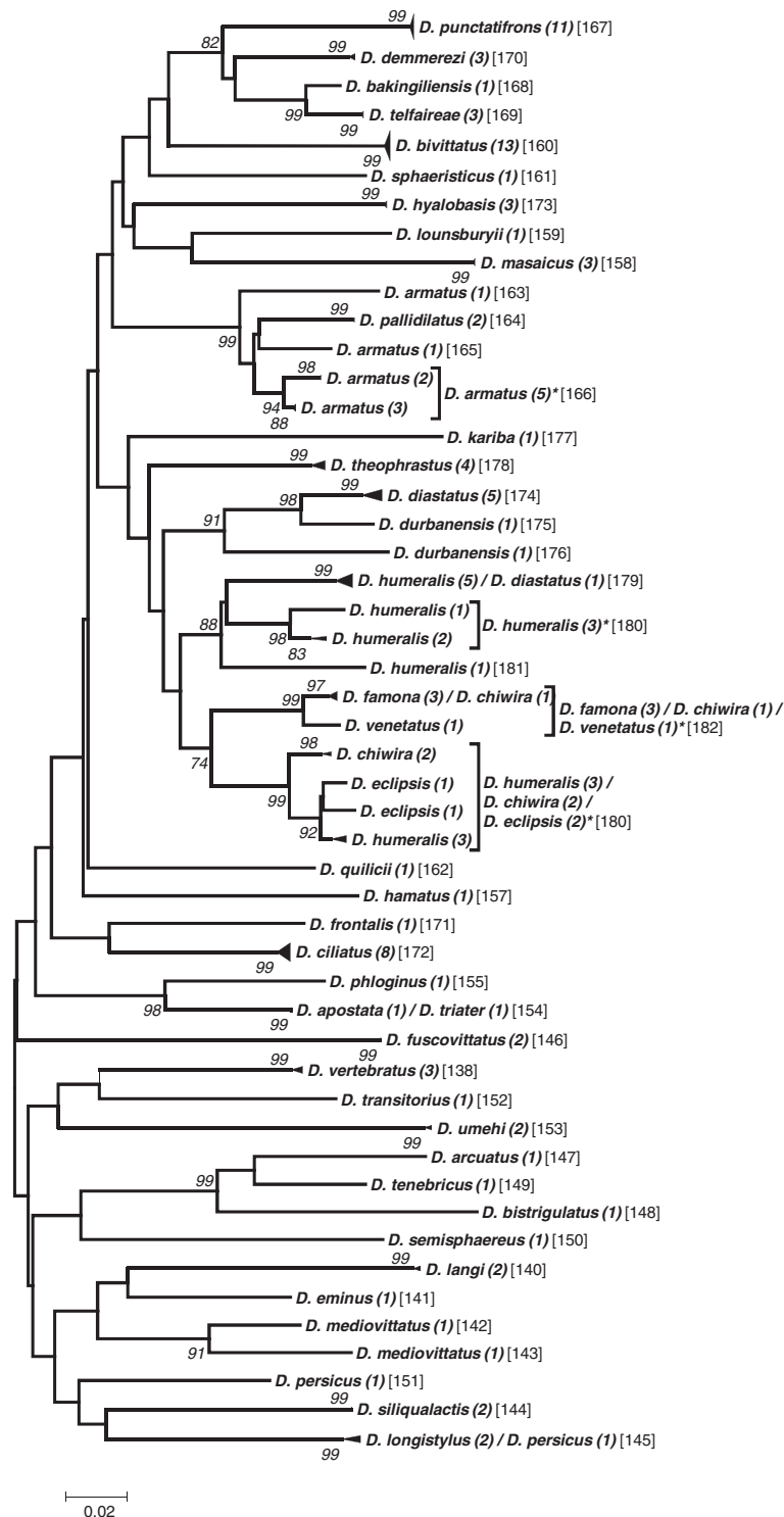
Figure 5 Evolutionary relationships among Dacus species.
