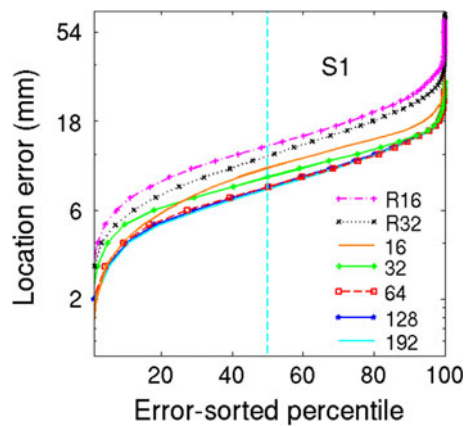
Fig. 16 Magnitude-sorted localization error distributions (subject S1) for source localizations performed using the sensor distributions shown in Fig. 14c–h and the wMNI-4 template head model
