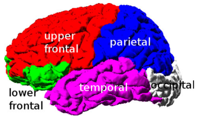
Fig. 17 Cortical regions of subject S1 brain. Segmentation obtained using FreeSurfer
