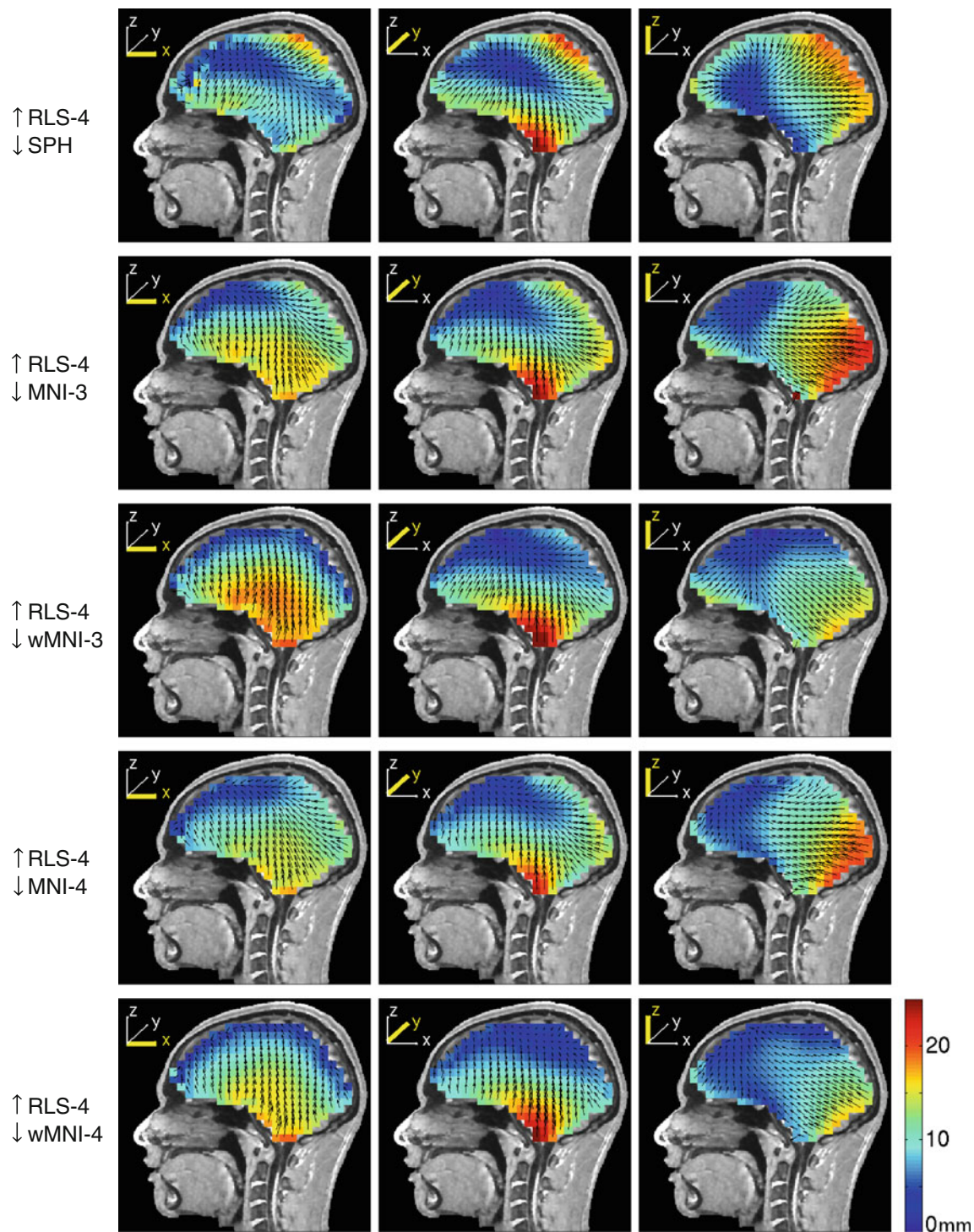
Fig. 4 Equivalent dipole source localization error directions ( arrows ) and magnitudes ( colors ) for spherical ( top row ) and four MNI-template based head models computed from source dipole scalp projections computed using a four-layer realistic subject MR image based BEM forward head model (subject S1 in Fig. 2). The forward and inverse models are indicated to the left of each row ( up arrow forward model, down arrow inverse model). The source space was a
