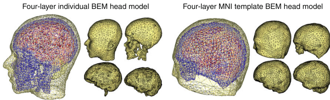
Fig. 1 A realistic head model generated from a subject T1-weighted whole head MR image ( left ) and an MNI template model fit to the same (subject S1) head ( right ). The four shells of the BEM models (scalp, skull, CSF, and grey matter) are shown to the right of each model
