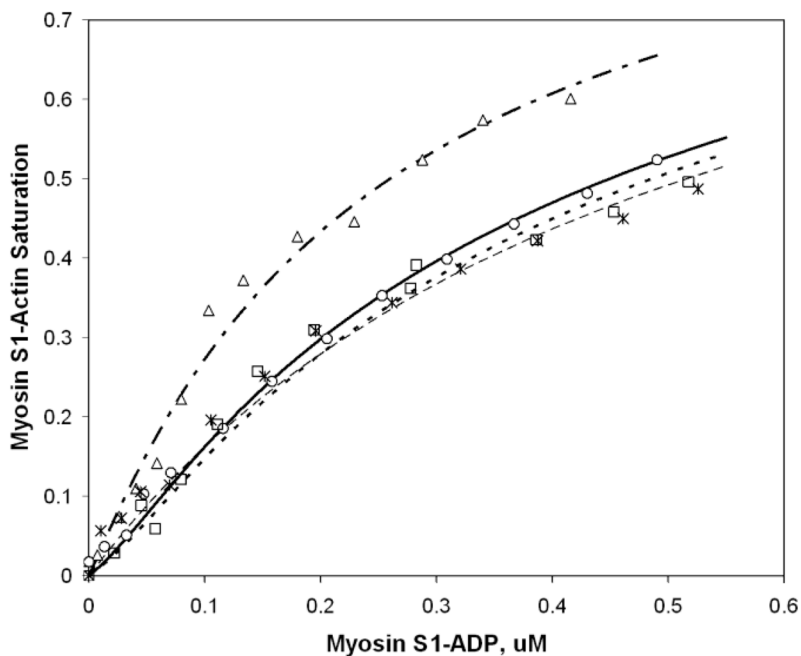
FIGURE 6. Chimera 3 tropomyosin enhances the affinity of myosin S1-ADP for the thin filament
