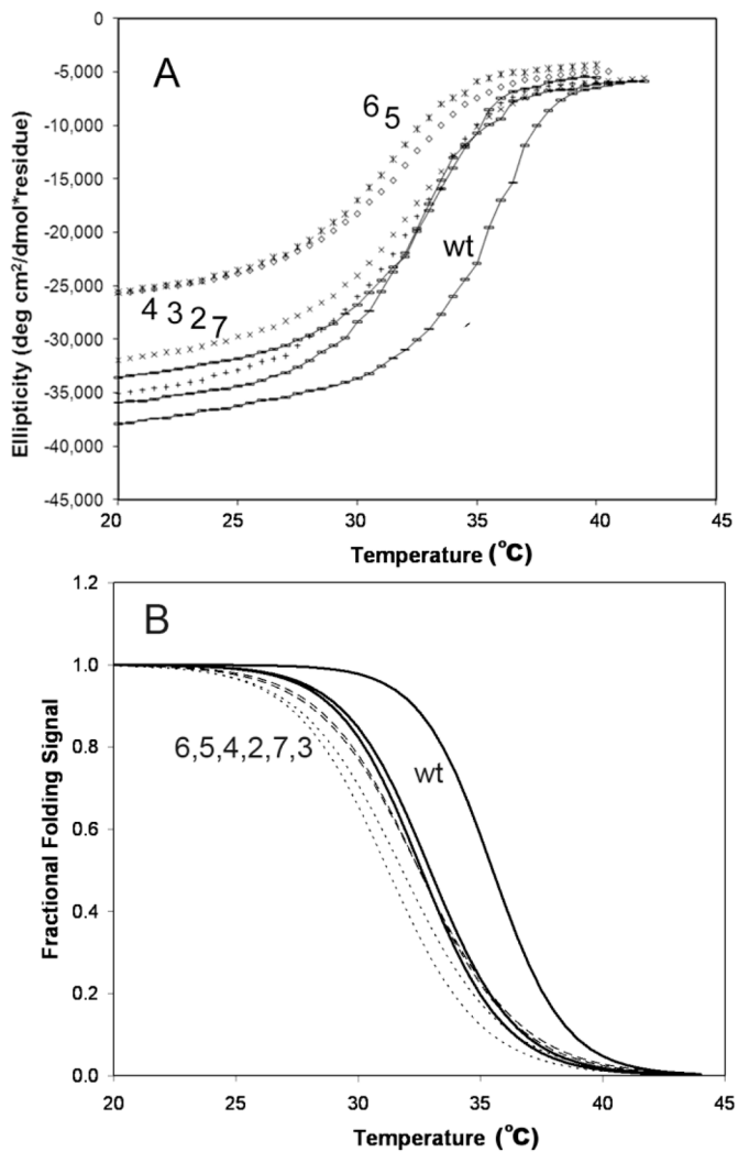
FIGURE 3. Thermal stability of chimeric tropomyosins assessed by circular dichroism A, ellipticity at \lambda=222 nm of wt TPM1 and chimeric tropomyosins 2, 3, 4, 5, 6, and 7 as a function of temperature. B, Two state thermal melting curves corresponding to best fits the data in Panel A, using parameters listed in Table 1. All of the chimeras had reduced stability. Note that data for chimeras 3 and 7 most resemble data for wt TPM1.
