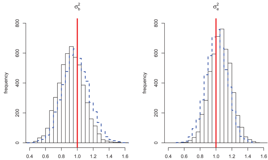
Figure 5. Distribution of Variance Component Estimates under the null hypothesis of no SNP Set effect: histograms with solid, black borders are for estimates computed using non-random selection of families (ascertained according to disease status), while the overlaid histograms in dashed-blue are for estimates computed using random selection of families. True parameter values are indicated by vertical red lines.
