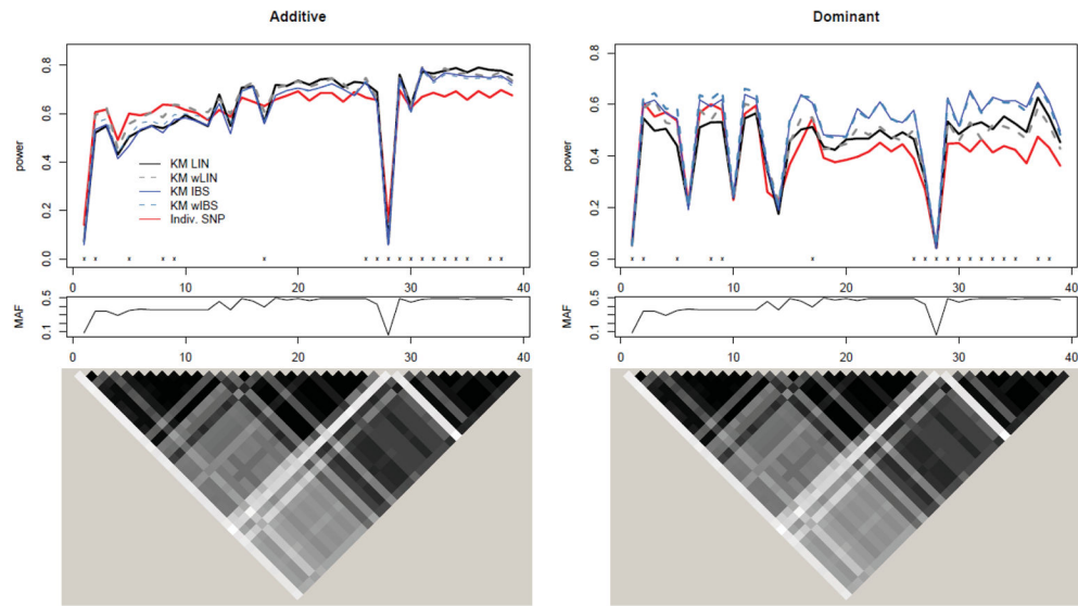
Figure 3. Power to detect causal SNP for ASA11 using additive (left) and dominant (right) genetic models under MED heritability due to SNP ( \max(h^2)=1\% ). Legend is the same as Figure 2.
