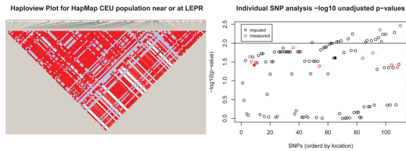
Figure 8. LD plot (standard D'/LOD color coding) using HapMap CEU population for the SNPs in the SNP set (left) and the individual-SNP analysis -\log_{10} unadjusted p-values for the GENOA dataset, ordered by SNP location (right). The solid, filled-in circles, indicate the previously published 'lead' SNPs.
