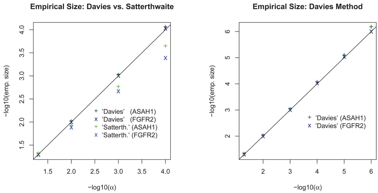
Figure 1. Empirical size for KM test (linear kernel) using Davies and Satterthwaite's Method and N=10^7 simulated datasets.
