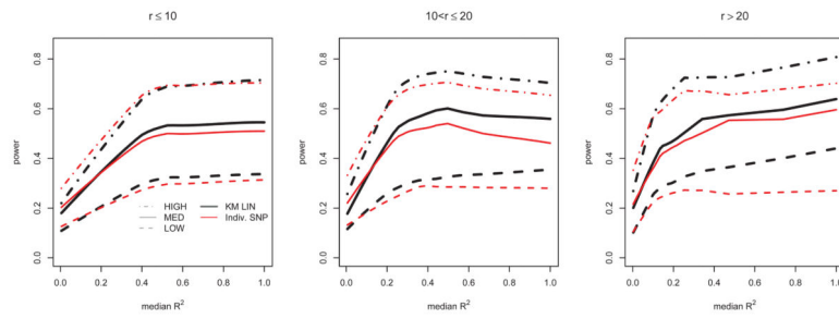
Figure 7. Power from Chromosome 10 simulation, plotted as a function of median R^2 for differing ranges of total number of SNPs in the SNP set ( r ). Different line types correspond to LOW, MED, and HIGH heritability due to SNP ( h^2 ).
