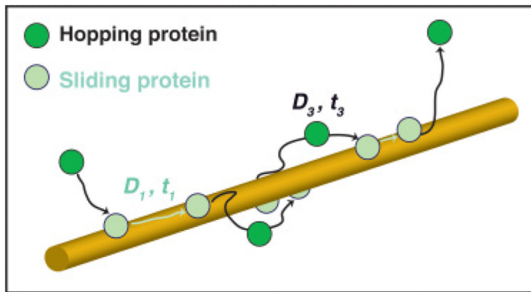
FIG. 1. (Color online) Schematics of a diffusion trajectory showing a protein initially binding to DNA, proceeding to slide (light disks) and hop (dark disks), and finally permanently dissociating from DNA. This example diffusion trajectory has two discernible hops.
