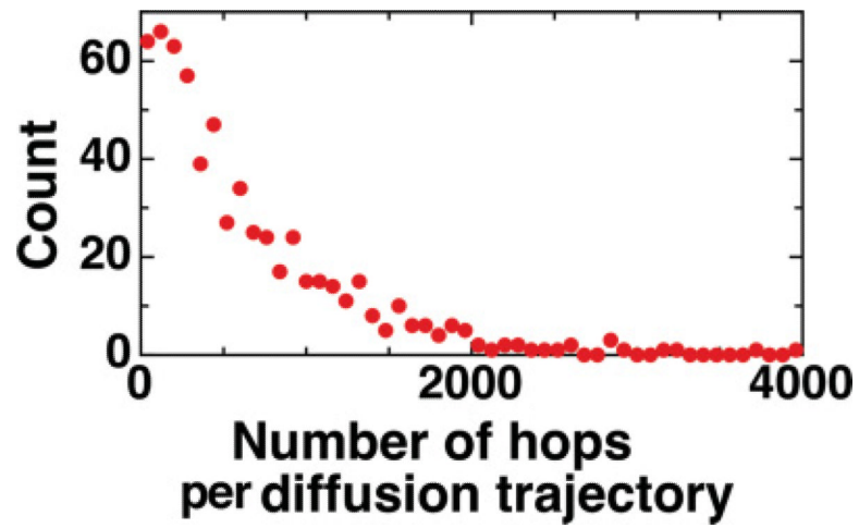
FIG. 4. (Color online) Distribution of number of hops per diffusion trajectory. The results of 4 \times 10^5 individual hopping simulations constitute a total of 763 protein diffusion trajectories such that 526 hops occur on average per trajectory.
