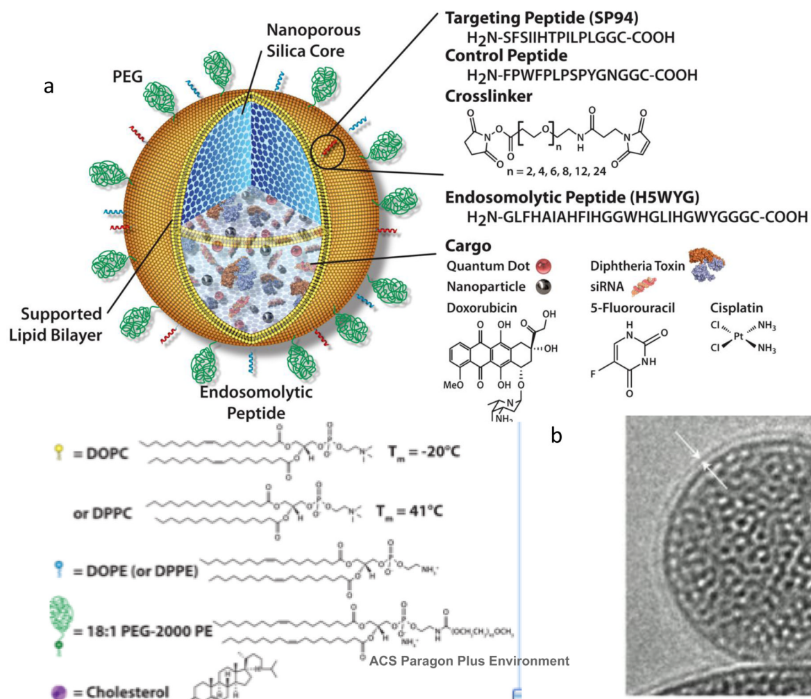
FIGURE 4. Schematic (a) and cryo-TEM image (b) of protocells.
