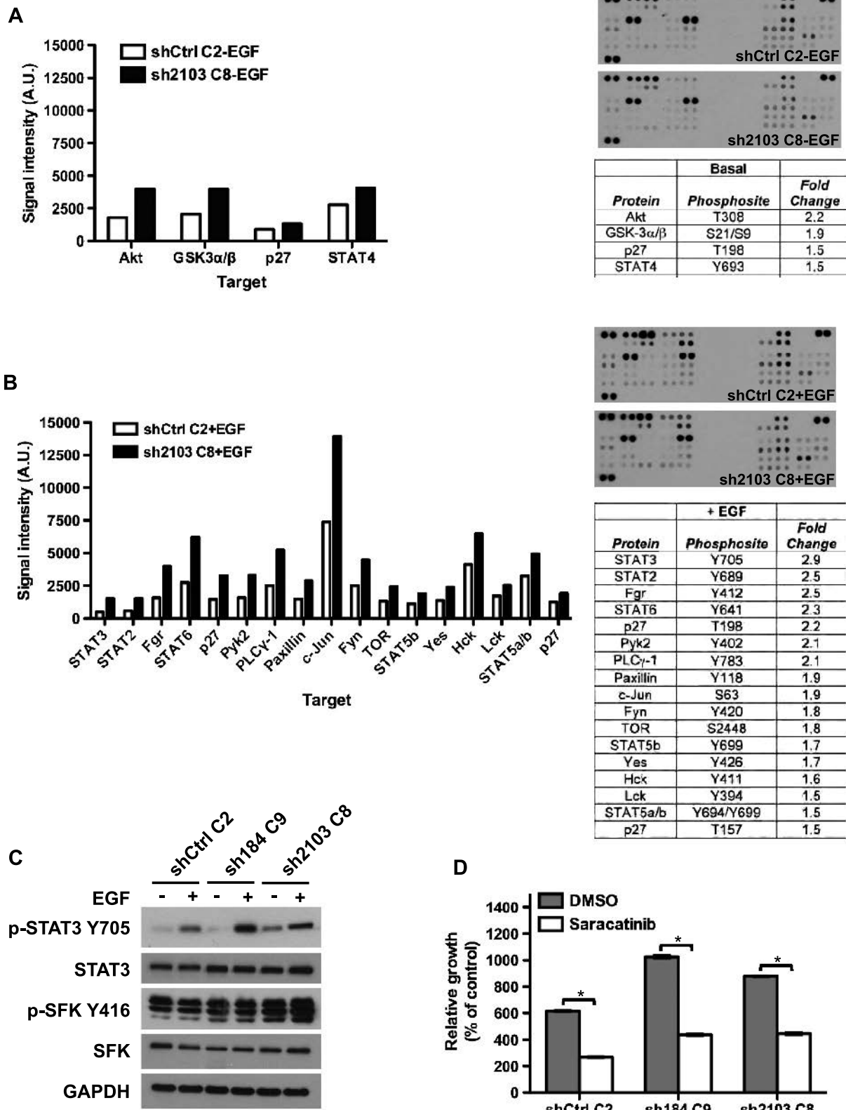
Figure 5. Stable Sh3gl2 silencing increases phosphorylation of SFKs and STAT3. Lysates of control and Sh3gl2-silenced cells treated without (A) or with (B) 10 nM EGF for 10 minutes were analyzed using a phospho-kinase proteome array. Graphs and tables indicate phosphoproteins that were altered by >1.5-fold in response to Sh3gl2 silencing. Representative images of phospho-array blots from each condition are shown. (C) Independent lysates immunoblotted with the indicated antibodies revealed enhanced phosphorylation of SFKs at Y416 (or corresponding conserved residue) and STAT3 at Y705. (D) Control and Sh3gl2-silenced RT4 cells were treated with vehicle (DMSO) or 0.125 μM saracatinib for 5 days and cell number determined by biomass assay. Graphs illustrate absorbance on day 5 expressed as a percentage of absorbance on day 0, and data are the means ± SD of two values for DMSO and six values for saracatinib. Data are representative of at least two independent trials. *P < .05 compared to DMSO-treated condition.
