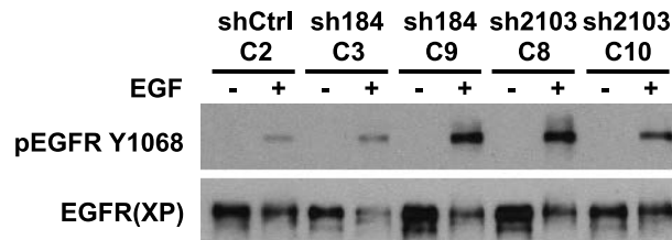
Figure W2. The figure shows independent evaluation of total EGFR levels in Sh3gl2-silenced RT4 clones and control RT4 cells treated with EGF, using a different anti-EGFR antibody from that used to generate data in Figure 4. Although signal avidity is lower following EGF treatment, consistent with modification of antibody epitopes following EGFR cytoplasmic domain phosphorylation, total EGFR is evident in all four Sh3gl2-silenced RT4 clones and control RT4 cells in the absence or presence of EGF treatment. On the basis of these findings, we conclude that Sh3gl2 silencing in RT4 cells leads to enhanced phosphorylation of the EGFR.
