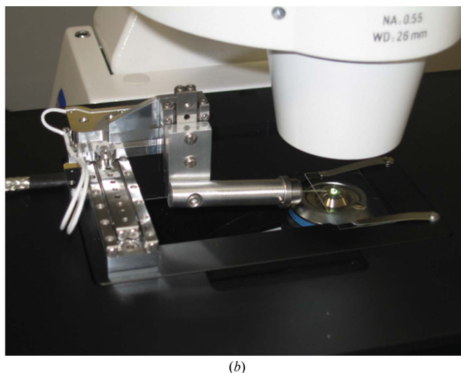
Figure 1 PALM MicroTweezers microscope (Zeiss). (a) Overall view. (b) Sample environment with SmarAct micromanipulators for sample holders.
