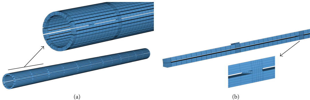
FIGURE 2: FE model of the slotted tube: (a) global model, (b) detail of knot between struts.
