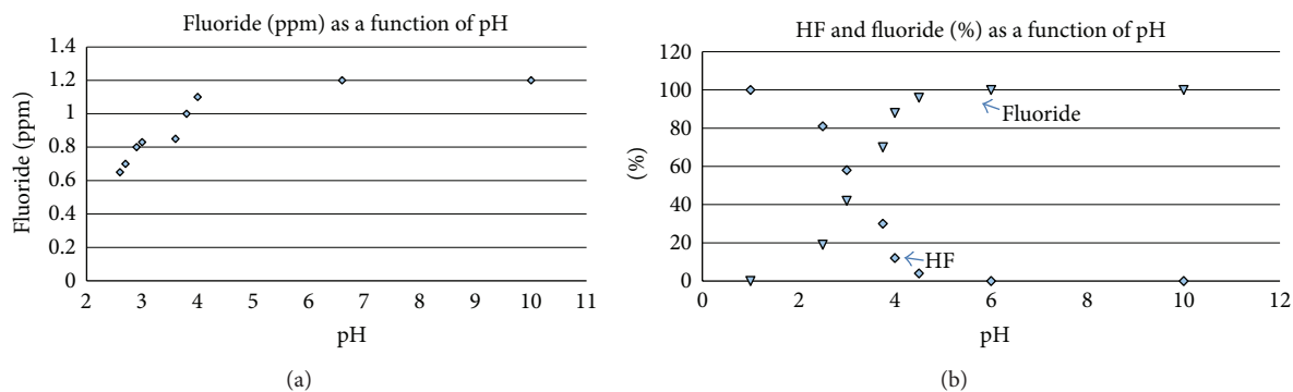
FIGURE 2: Fluoride protonation depends on prevailing acidity following the equilibrium reaction F^- + H^+ \leftrightarrow HF . (a) All measurements of fluoride ion concentration were made with a LaMotte Instruments fluoride ion specific electrode calibrated with a 1.00 ppm fluoride standard solution in distilled deionized water at room temperature. Readings for the 1.2 ppm true concentration solution progressively decrease as pH decreases. Acidity was adjusted with dilute acetic acid. Stomach acid pH normally varies from 1.5 to 3 (Teitz [18] p. 1072), where fluoride is mostly protonated as hydrofluoric acid HF. (b) The percent contribution to the total fluoride from the free ion F^- (triangles) and intact HF (diamonds), calculated theoretically from the Henderson Hasselbach equation pH = pK_a + \log\{[F^-]/[HF]\} over the pH range 1–10, utilizing the known K_a for HF. HF decreases while F^- increases from pH 1 to 5. At pH 3.14 ( = pK_a = -\log 7.2 \times 10^{-4} ), HF is half dissociated.
