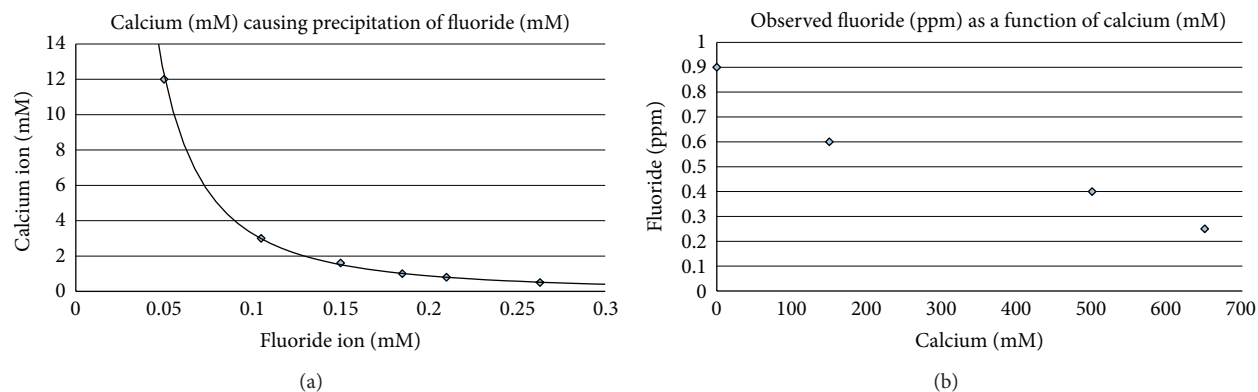
FIGURE 1: (a) Calcium concentrations (mM) that precipitate various fluoride concentrations. From the known solubility product constant K_{sp} for calcium fluoride, the calculated isocurve for \text{CaF}_2 precipitation is shown as a function of varying concentrations for the two ions. Calcium levels in normal blood (1–3 mM) reach precipitation maximum solubility with 0.1–0.18 mM (1.9–3.4 ppm) fluoride. For 3 mM calcium, precipitation begins to occur when fluoride is 3% of calcium and for 1 mM at 18%. The Hooper Bay poisoning incident produced a lethal 5 ppm blood fluoride level in one victim. Whether it is a low Ca/F ratio or rather calcium fluoride saturation that is required for acute toxicity is not known. (b) Calcium effects on measured fluoride ion concentration. A 0.9 ppm fluoride solution in distilled water was measured for free fluoride ion level with a LaMotte fluoride specific electrode calibrated with 1.00 ppm sodium fluoride in distilled deionized water at room temperature. Calcium ion was adjusted over a wide range by addition of aliquots of calcium biphosphate. Fluoride readings progressively decrease with increasing calcium concentration as expected over the range 30–650 mM.
