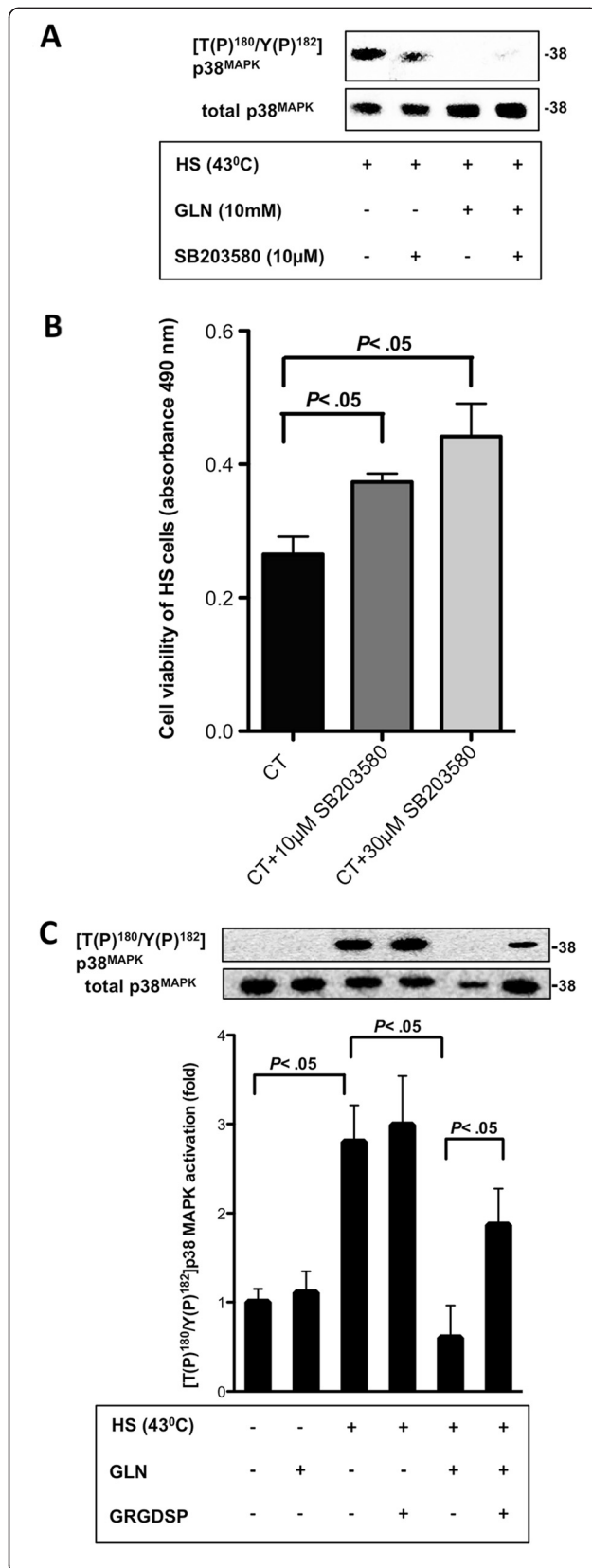
Figure 3 GLN is protective by dephosphorylating p38MAPK downstream of GLN-mediated FN-Integrin osmosignaling after HS. A ) Cells were treated with 0 mM or 10 mM GLN with or without SB203580 (10 µM) 1 h prior treatment under stressed conditions (43°C). A representative Western blot of [T(P) 180 Y(P) 182 ]p38MAPK and total p38MAPK levels is shown. B ) IEC-6 cells were treated with/without 1 h prior SB203580 (10 µM and 30 µM) treatment under stressed conditions (44°C). Cell survival was measured via MTS assay. Results are shown as mean ± SEM (n = 4). C ) IEC-6 cells were treated as described in Figure 2A. Western blots of [T(P) 180 Y(P) 182 ]p38MAPK and total p38MAPK levels are shown. P38MAPK phosphorylation is revealed as mean fold change relative to total p38MAPK ± SEM and ratioed to 0 mM GLN (n = 4).
