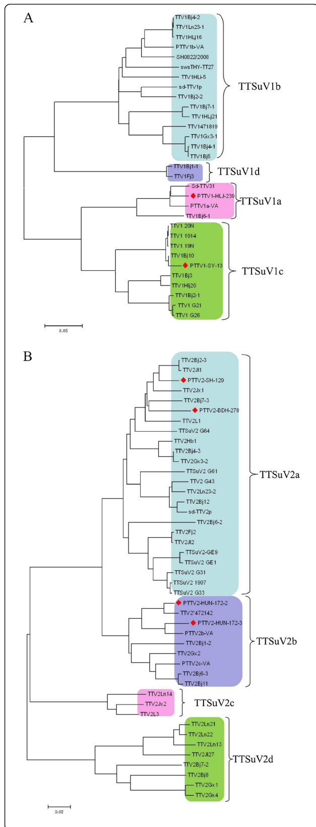
Figure 1 Phylogenetic tree constructed by the neighbor-joining method based upon the full-length genomic nucleotide sequences of the TTSuV strains. (A) Phylogenetic trees based on 31 full-length sequences of TTSuV1, including 2 strains isolated in this study and 29 strains submitted to GenBank. (B) Phylogenetic trees based on 44 full-length sequences of TTSuV2, including 4 strains isolated from this study and 40 strains submitted to GenBank. The tree was constructed using a neighbor-joining algorithm with the MEGA4.0 software. The red color indicates the strains that were isolated in this study.
