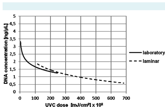
FIGURE 5. The correlation between DNA concentration values and doses of UVC radiation for the experiments performed in the laboratory and laminar using 10 \mu\text{L} of undiluted semen treated only with UVC radiation (only-UVC group).
