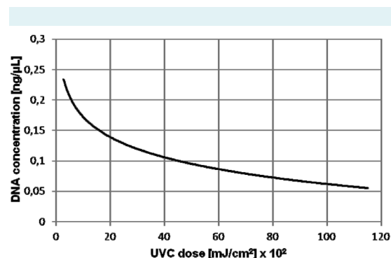
FIGURE 2. The correlation between DNA concentration and doses of UVC radiation for the experiments performed in the laboratory and laminar using 10 μL of undiluted saliva treated only with UVC radiation (only-UVC group).
