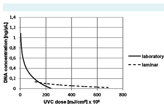
FIGURE 1. The correlation between DNA concentration and doses of UVC radiation for the experiments performed in the laboratory and laminar using 10 μL of undiluted blood treated only with UVC radiation (only-UVC group).
