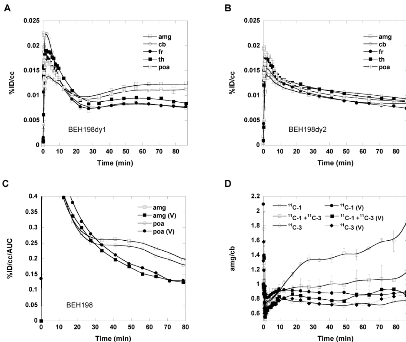
Fig 5. Comparison of time-activity curves for [ N -methyl- 11 C]vorozole in the baboon brain over a 90 minute scanning session at (A) baseline ( 11 C-1, 163.91 MBq (4.43 mCi)), (B) after treatment with vorozole (0.1 mg/kg, 5 min prior) ( 11 C-1, 173.16 MBq (4.68 mCi)), (C) time-activity curves for amygdala and preoptic areas corrected for the area under the plasma time-activity curves (AUC) at baseline (open symbols) and after pretreatment with vorozole (closed symbols). (D), ratio of amygdala/cerebellum vs time for 11 C-1 (n=3), mixture ( 11 C-1 + 11 C-3, n=2), and N-3 isomer ( 11 C-3, n=1) at baseline and after pretreatment with vorozole in baboons. Abbreviations are amygdala (amg), cerebellum (cb), frontal cortex (fr), thalamus (th), preoptic area (poa); V (vorozole).
