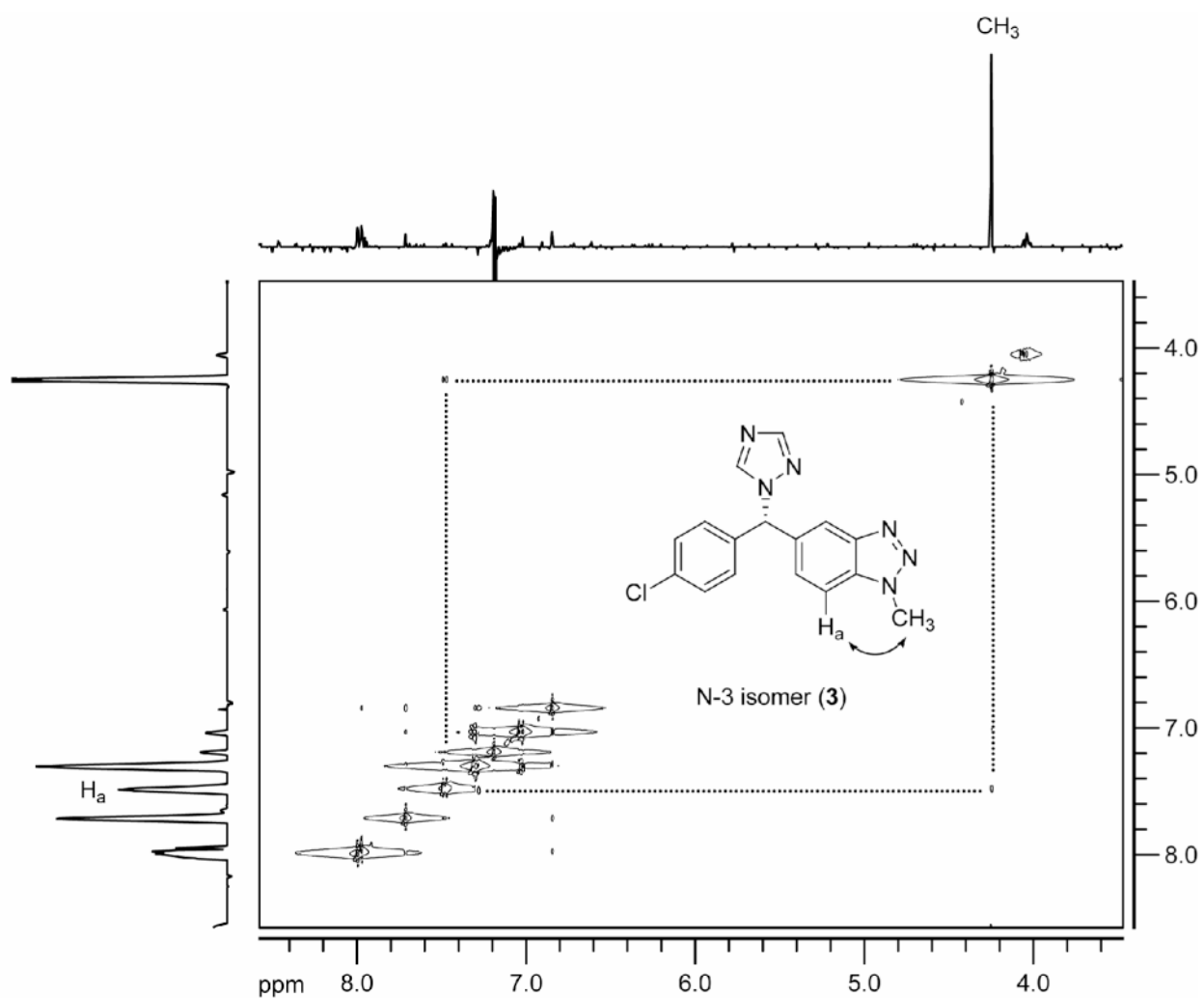
Fig 1. The 2D-NOESY spectrum of N-3 isomer ( 3 ) acquired in CDCl 3 at 400 MHz.
