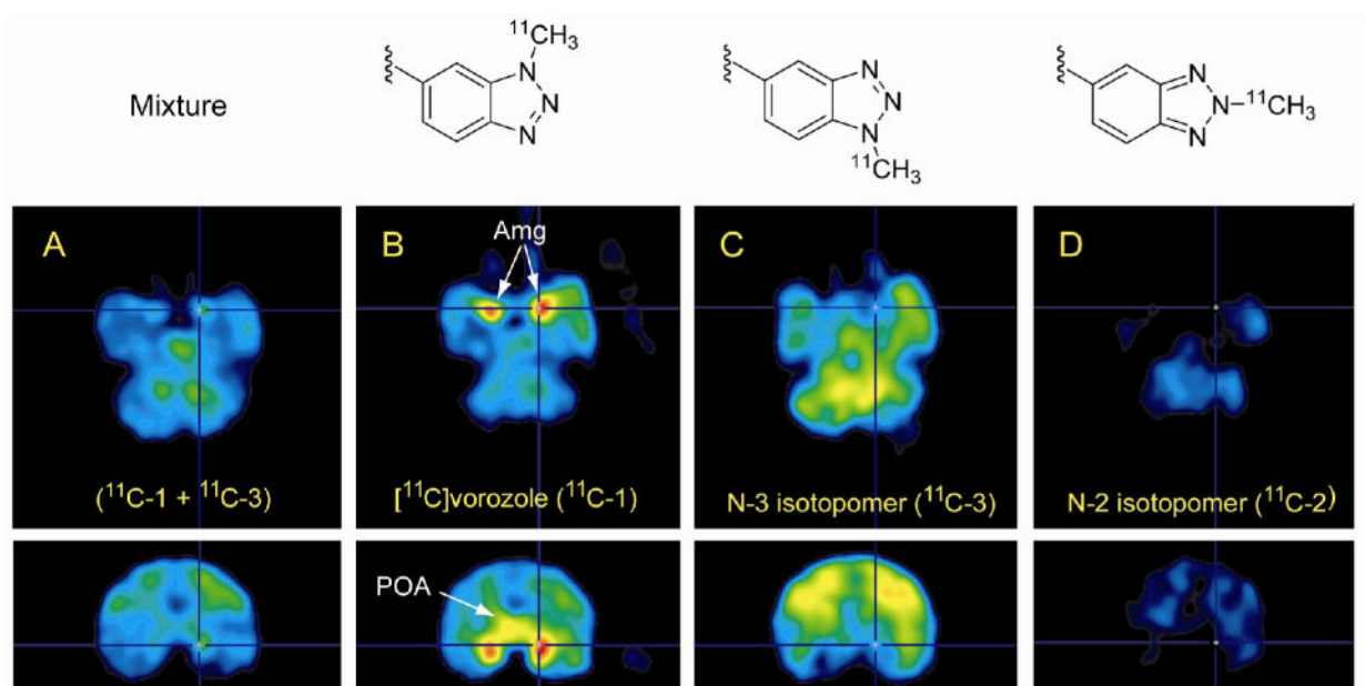
Fig 4. PET images in the (transaxial (top row) and coronal (bottom row) planes in baboon brain summed from 15-90 min after injection for (A) the 15 minute fraction (X), ( ^{11}\text{C-1} + ^{11}\text{C-3} , 176.49 MBq (4.77 mCi)), (B) [N-methyl- ^{11}\text{C} ]vorozole ( ^{11}\text{C-1} , 163.91 MBq (4.43 mCi)); (C) N-3 isomer ( ^{11}\text{C-3} , 123.21 MBq (3.33 mCi)) and (D) N-2 isomer ( ^{11}\text{C-2} , 44.77 MBq (1.21 mCi)). All PET images are dose-corrected. Arrows indicate the amygdala (Amg) and preoptic area (POA).
