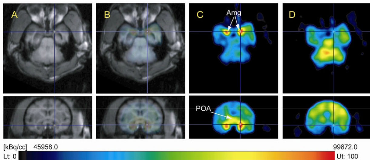
Fig 6. Comparisons of [ N -methyl- ^{11}\text{C} ]vorozole ( ^{11}\text{C} -1) PET images in the same baboon brain in transaxial (top row) and coronal (bottom row) view between baseline and pretreatment with vorozole ( 1 ). (A), MR images; (B) coregistered ^{11}\text{C} -1 PET and MR images; (C), [ N -methyl- ^{11}\text{C} ]vorozole ( ^{11}\text{C} -1, 163.91 MBq (4.43 mCi)) PET images; (D), PET images following pretreatment with vorozole (0.1 mg/kg) 5 min before the injection of [ N -methyl- ^{11}\text{C} ]vorozole ( ^{11}\text{C} -1, 173.16 MBq (4.68 mCi)). Amg, amygdala; POA, preoptic area. All PET images were summed over 15-90 min and PET image (D) was dose-corrected based on (C).
