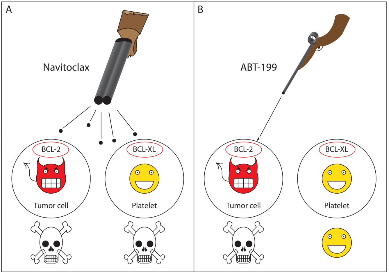
Figure 1. ABT-199 selectively kills BCL-2 dependent tumor cells while sparing platelets (A) Navitoclax (ABT-263) binds with high affinity to both BCL-2 and BCL-XL. Since many tumors, particularly lymphoid malignancies, are addicted to BCL-2 for survival, this potently induces tumor cell apoptosis. Platelets depend primarily on BCL-XL for survival, and therefore are also destroyed by navitoclax. (B) ABT-199 is specific for BCL-2 and induces selective death of BCL-2 dependent tumor cells while sparing platelets.
