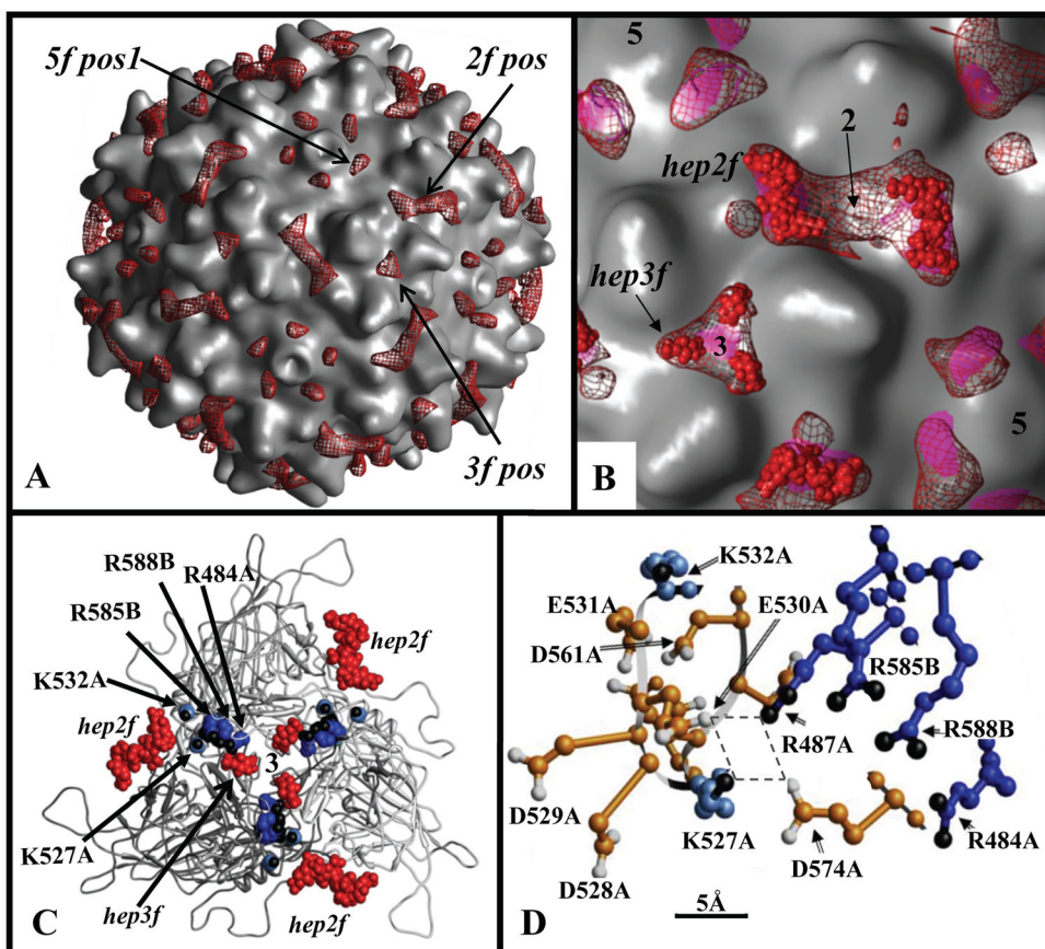
Figure 2. AAV2 crystal structure with superimposed AAV2-Hep minus AAV2 VLP positive difference map and heparin models. (A) Shaded-surface electron density map of AAV2 (PDB accession No. 1LP3, Xie et al., 2002) (grey) with the positive density (red mesh, contoured at 1\sigma ) close to the two-, three-, and fivefold axes, 2f pos , 3f pos and 5f pos1 , respectively, superimposed. (B) Close-up of shaded-surface representation of VLP reconstruction (grey) and AAV2-Hep (pink, density not in present VLPs), with the pseudo-atomic coordinates of heparin oligosaccharides (solid red) modeled into positive density (red mesh). hep2f = decasaccharide (twofold symmetry related decasaccharide is also shown); hep3f = single disaccharide (threefold symmetry related models are also shown). (C) Ribbon diagram of an AAV2 VP3 trimer and modeled heparin molecules. Surface heparin binding residues, R484, K527, K532, R585, and R588, are shown in blue (Arginines) or light blue (lysines) with terminal amino groups depicted as black balls. Residues from a reference monomer are denoted with A after the residue number; B indicates a threefold related residue. Heparin models are as labeled in (B). (D) Close up of basic (blue), acidic (orange) residues flanking the heparin binding residues. Basic residues are colored as in (C) and carboxyl groups are white for acidic residues. The broken lines indicate potential ionic interactions. The location of the icosahedral symmetry axes are labeled with numbers in (A–C). (A) is viewed along a twofold axis, and B, C, and D along a threefold axis. The figure was generated using Chimera (Pettersen et al., 2004).
