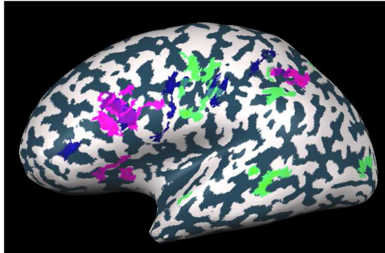
Figure 1. Statistical parametric map of 20 subjects using random effect GLM analysis ( p < 0.05 , cluster size corrected) for the different conditions. The three maps overlaid (semantic – green, orthographic – blue, morphological – pink) on an inflated brain of one subject, presented from a lateral view.
