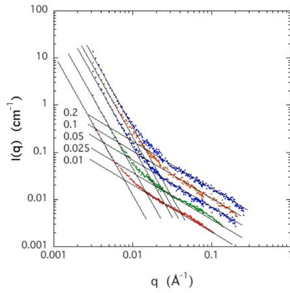
Figure A1. Power law fits to SANS spectra at different CS concentrations 100 mM NaCl.
