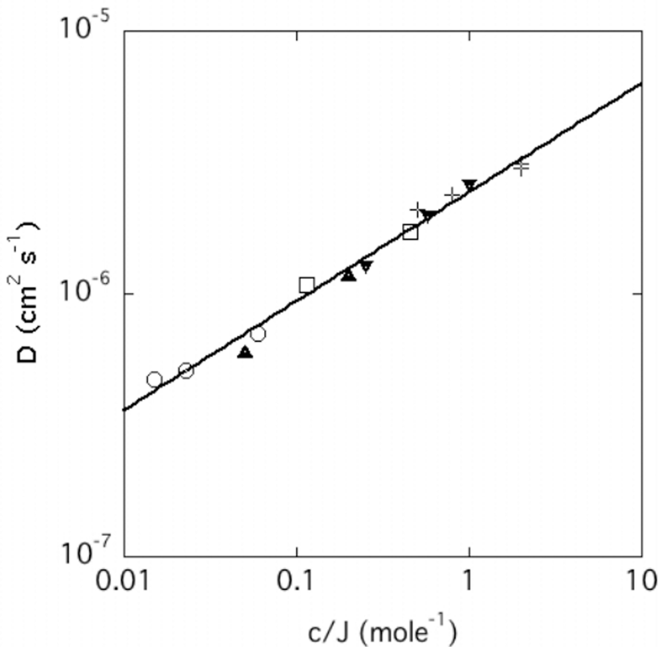
Figure 8. Dependence of D on the variable c/J , where c is expressed in mass fraction w/w, J is the ionic strength in moles. Symbols: ○ : c = 0.006 ; up triangles: c = 0.02 ; open square: c = 0.046 ; down triangle c = 0.1 ; + c = 0.2 .
