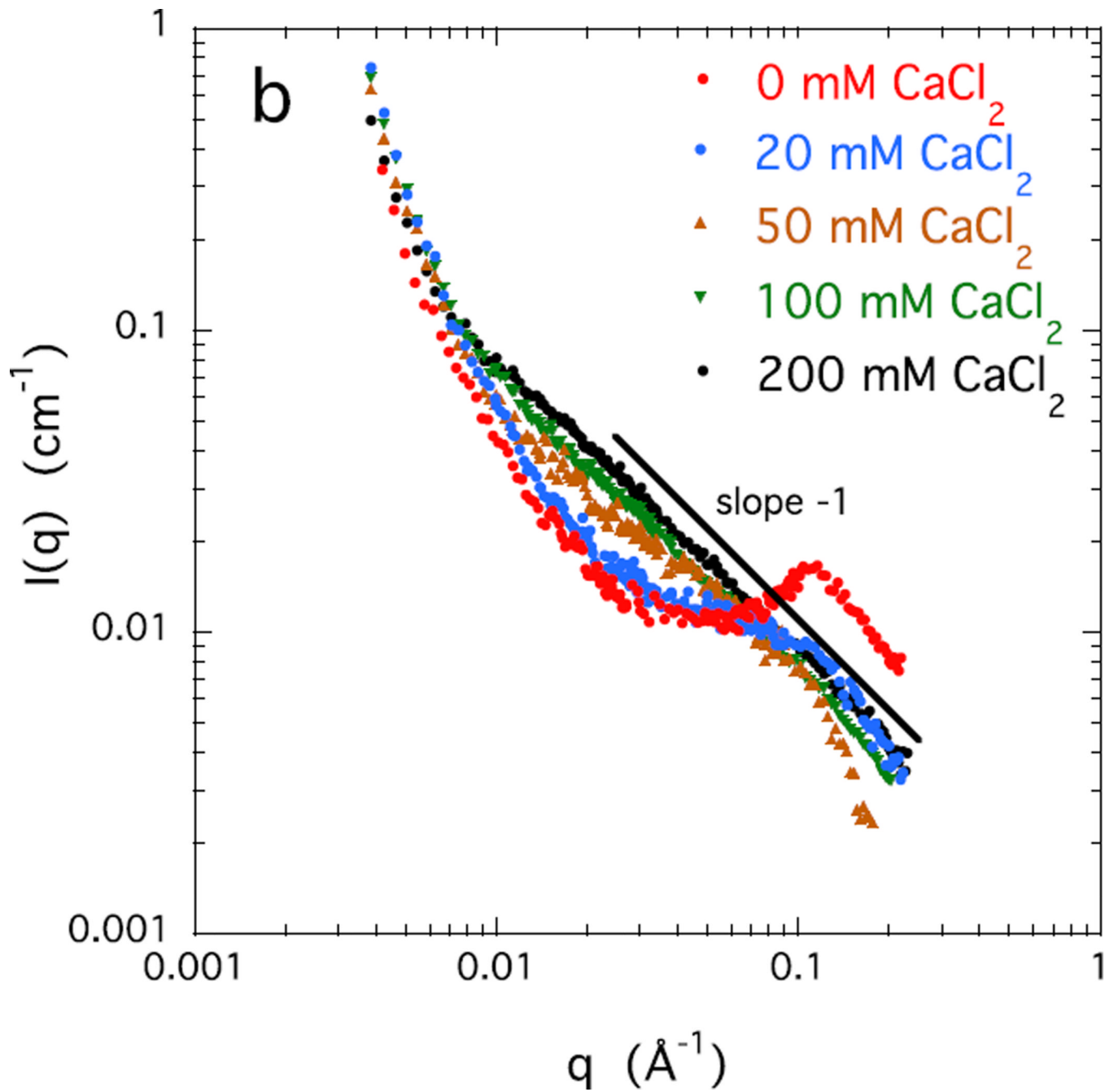
Figure 3. SANS response of 4% w/w CS solutions at different concentrations of a) NaCl, and b) \text{CaCl}_2 .
