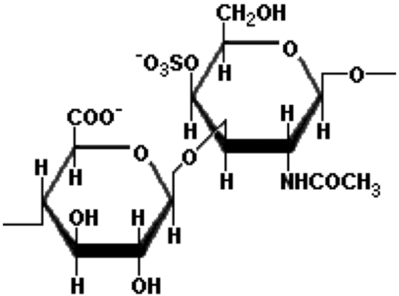
Figure 1. Chemical structure of the disaccharide repeating unit of the CS chain.
