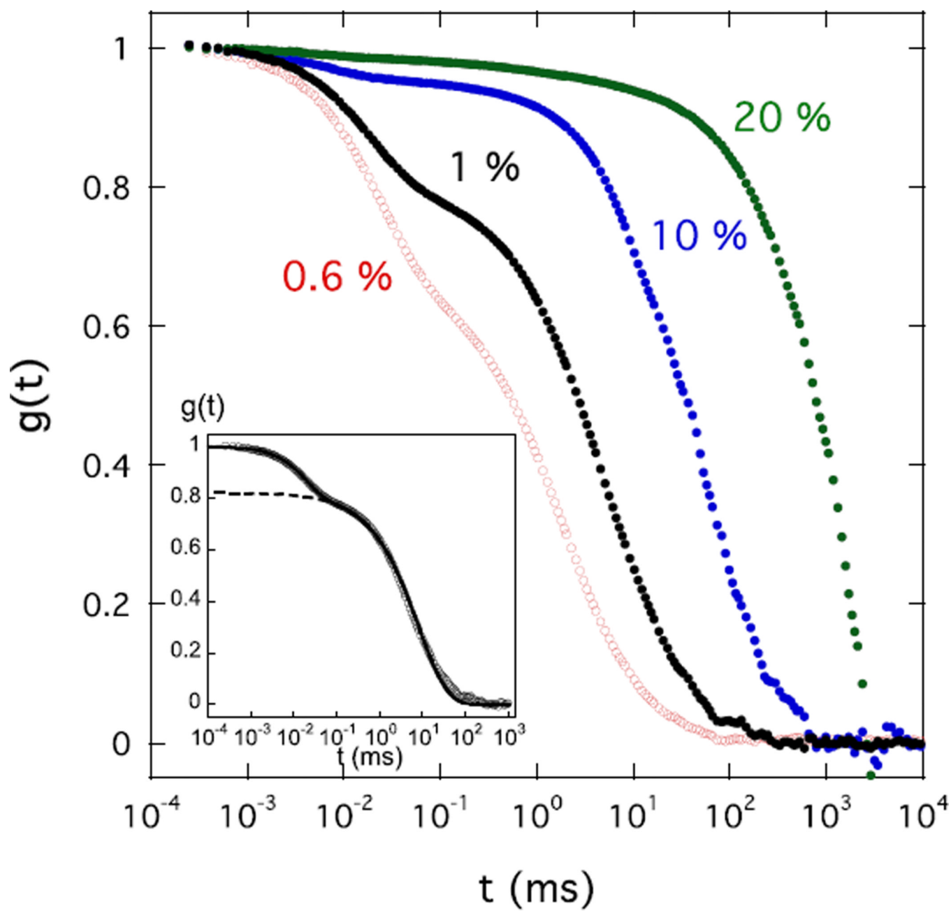
Figure 5. Field correlation functions g(t) of light scattered at \theta = 150^\circ by CS solutions of different concentration c in 100 mM NaCl. Inset shows fit of eq 3 to the data from c=1\% w/w (continuous line); dashed line is the second term in the fit to this equation.
