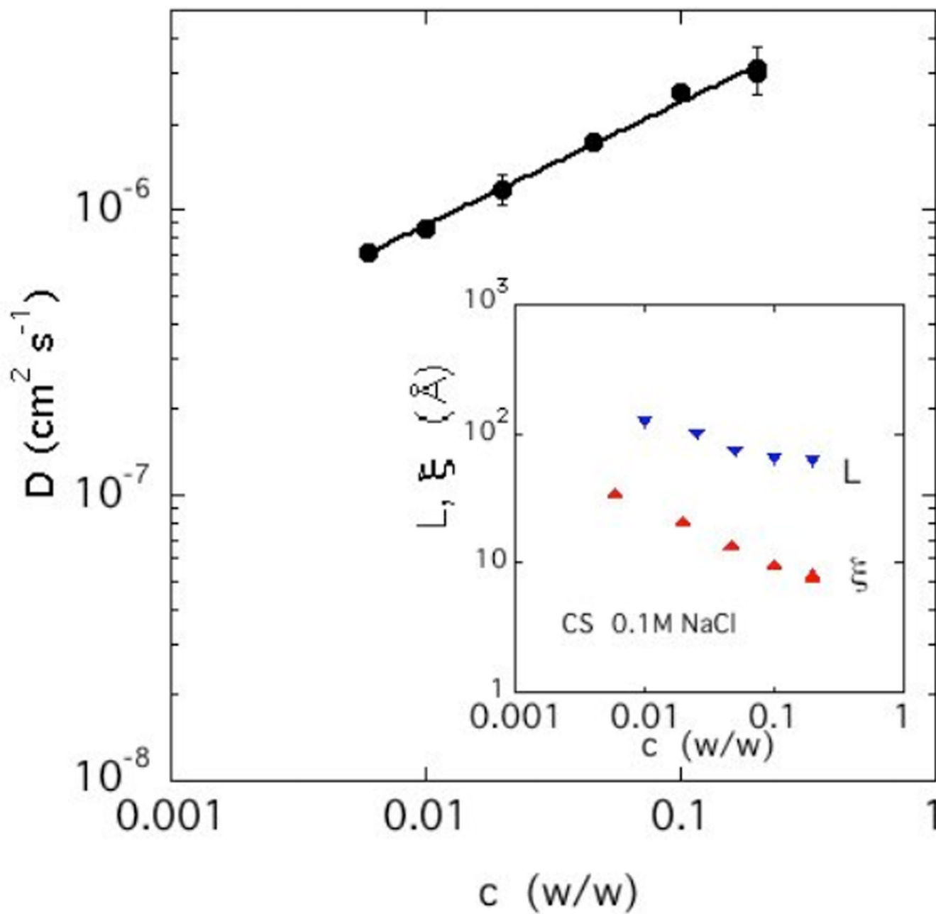
Figure 6. Dependence of D on CS concentration in solution with 100 mM NaCl. The slope of the power law fit is 0.43. Inset: characteristic linear range L from SANS and correlation length \xi from DLS.
