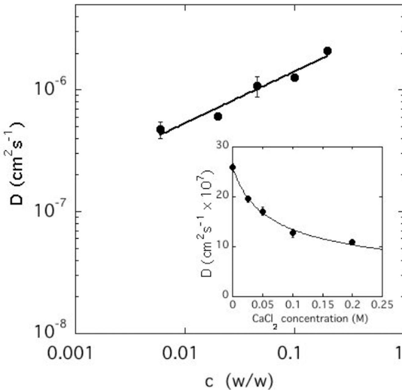
Figure 7. Variation of the collective diffusion coefficient D with concentration of CS solution in 100 mM NaCl + 100 mM \text{CaCl}_2 . Inset: variation of D with \text{CaCl}_2 concentration for c = 10\% w/w.
