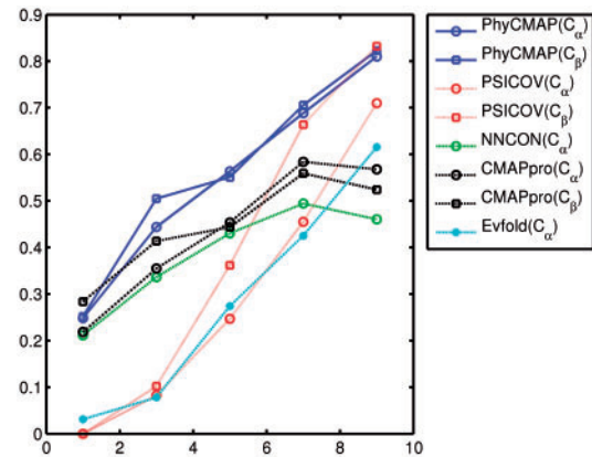
Fig. 4. The relationship between prediction accuracy and the number of non-redundant sequence homologs ( M_{eff} ). x -axis is \log M_{eff} and y -axis is the mean accuracy of top L/10 predicted contacts on the corresponding CASP10 target group. Only medium- and long-range contacts are considered
