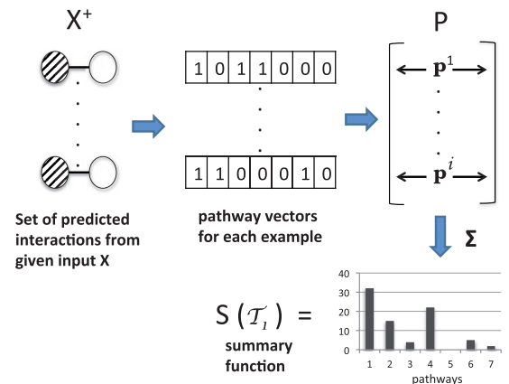
Fig. 2. A schematic illustrating the pathway summarizing function S for a task \mathcal{T}_1 . On the left are the examples from the input predicted to be positive, indicated by X^+ . The matrix P has the pathway vectors for each example in X^+ . The summary function aggregates the pathway vectors to get the distribution
