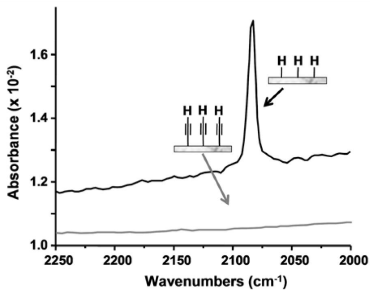
Figure 4. ATR-FTIR characterization of a H-[Si(111)] and H-C \equiv C-[Si(111)], in the region of the 2083 \text{cm}^{-1} Si-H mode.
