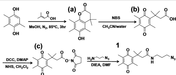
Scheme 2. Synthesis of electroactive benzoquinone 1.
