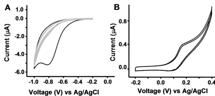
Figure 3. Cyclic voltammograms (CVs) for 1s and 3s . A) The electrochemical activation of 1s to 2s . The black trace is of the first scan, and the grey traces are of two subsequent scans, indicating nearly complete conversion of benzoquinone to hydroquinone during the first scan. B) The reversible oxidation of 3s . Two subsequent scans are shown. CVs were performed at a rate of 100 mV/s with voltages relative to Ag/AgCl.
