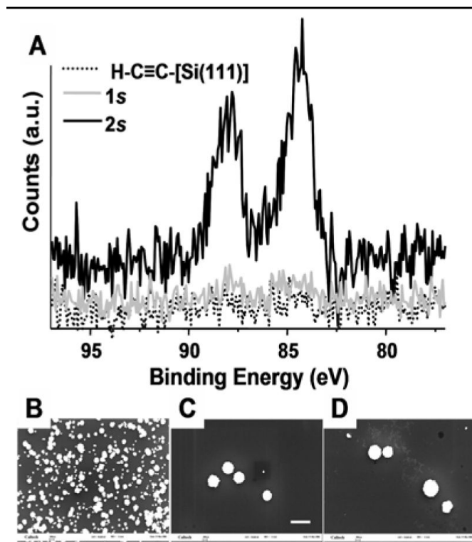
Figure 5. Demonstration of bioattachment to acetylenylated Si(111) through reductive formation of 2s followed by the amide coupling of biotin. A) XPS of the biotinylated Si(111) surface following exposure to strept-Au, but prior to the electroless Au amplification. The Au 4f region is comprised of two spin-orbit coupled peaks: Au 4f 7/2 (~84 BeV) and Au 4f 5/2 (~88 BeV). The dotted trace is from H-C≡C-[Si(111)], and the grey trace is from 1s , each exposed to biotin and strept-Au as controls. The three SEM images (B, C, and D) are of the activated and biofunctionalized surface, plus two controls. All images were taken following the electroless amplification step. The scale bar is 1 μm. B) 2s , incubated with biotin, and exposed to strept-Au. C) H-C≡C-[Si(111)] incubated with biotin, and exposed to strept-Au. D) 1s incubated with biotin, and exposed to strept-Au. There are at least 500 Au nucleation sites on B, 5 on C, and 7 on D.
