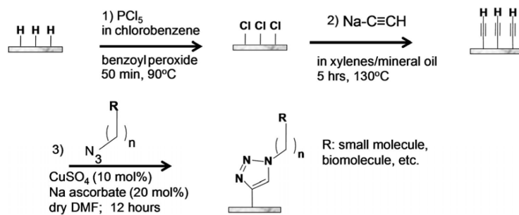
Scheme 1. Strategy for the functionalization of Si(111).
