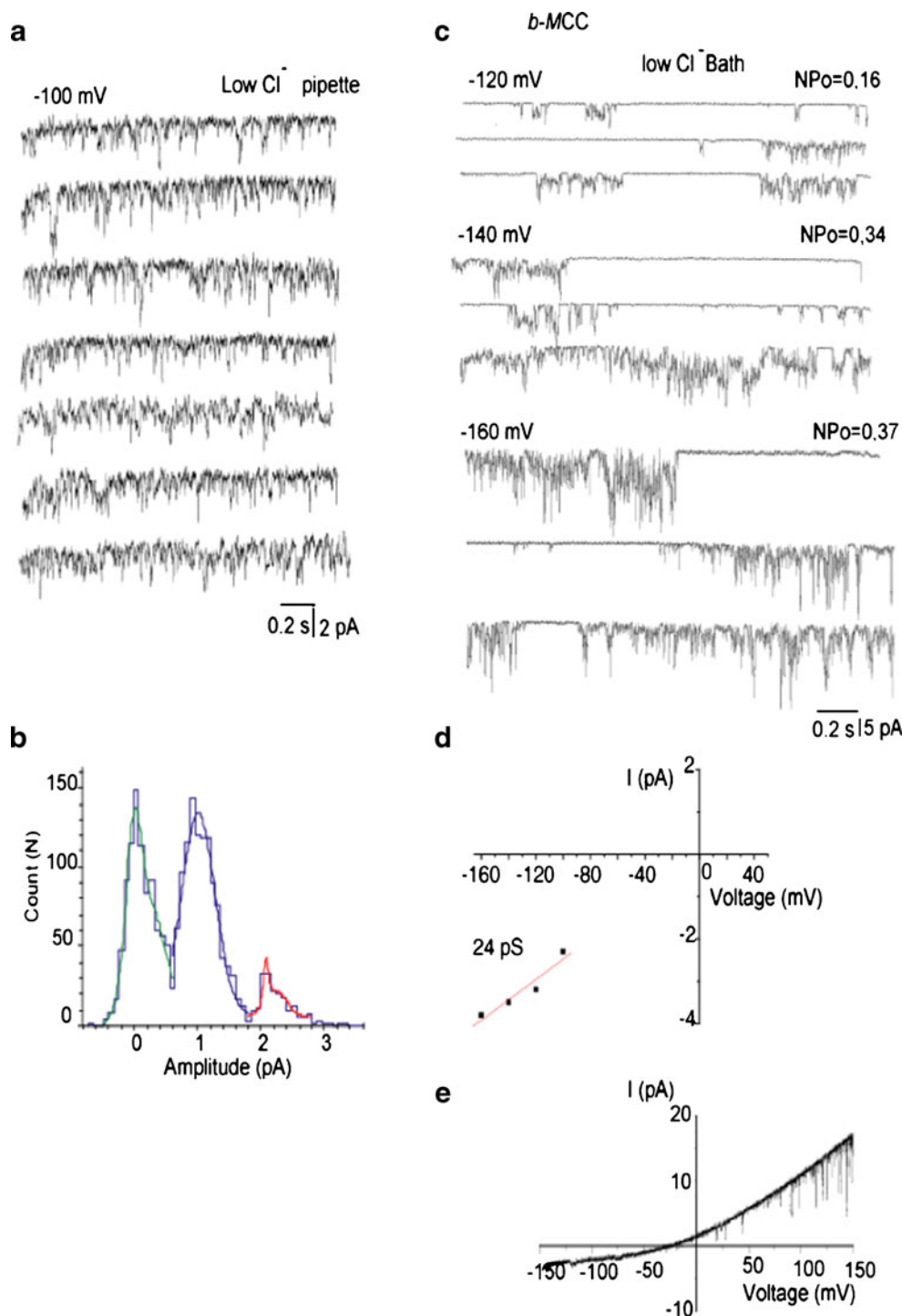
Fig. 9 Effect of manipulation of \text{Cl}^- concentrations on (\text{Ca}^{2+}) inward currents in mitoplasts. a Representative traces of i -MCC channel activity recorded with the use of low \text{Cl}^- (40 mM \text{Cl}^- )-containing pipette solution. Test potential is -100 mV. b Amplitude histogram of the channel activity shown in (a). c Representative traces showing the activity of b -MCC at different voltages indicated in the presence of 40 mM bath \text{Cl}^- . d Corresponding voltage dependency of single-channel openings shown in (c). e Representative current responses to a voltage ramps from -150 to +150 mV under our standard recording conditions showing the activity of \text{Cl}^- channels at positive potentials
