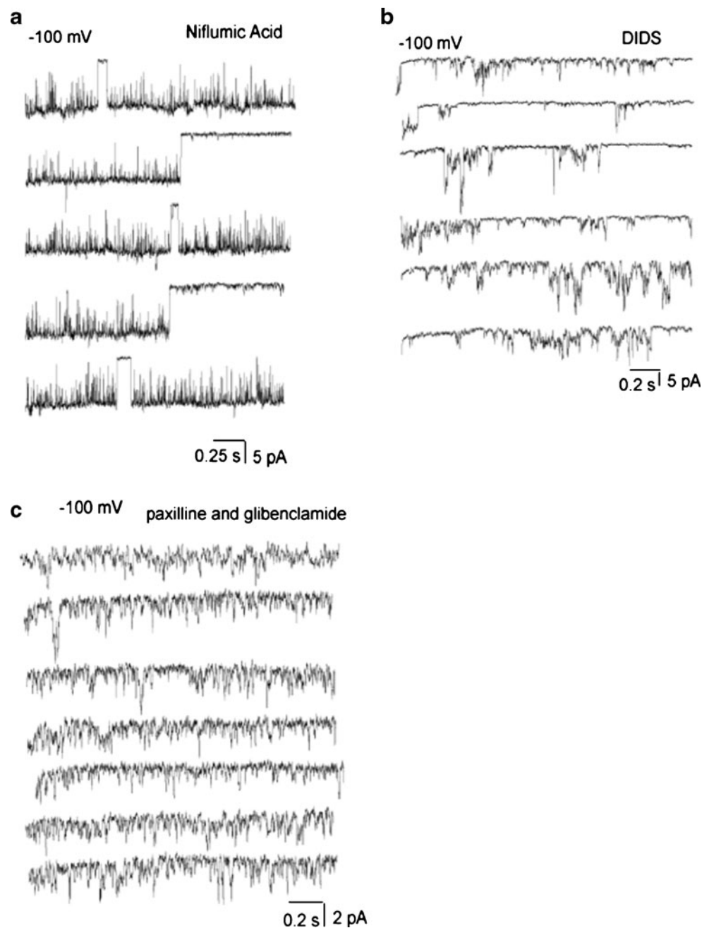
Fig. 10 Pharmacological characterization of ( \text{Ca}^{2+} ) inward currents in mitoplasts. a Representative traces showing x / l -MCC channel activity in the presence of 100 \mu\text{M} niflumic acid in the pipette solution. Test potential is -100\text{ mV} . b Representative traces showing the activities of b -MCC and i -MCC in the same patch in the presence of 100 \mu\text{M} DIDS in the pipette solution. Test potential is -100\text{ mV} . c Representative traces showing the activity of b i -MCC in the presence of 1 \mu\text{M} paxilline and 10 \mu\text{M} glibenclamide in the pipette solution. Test potential is -100\text{ mV}
