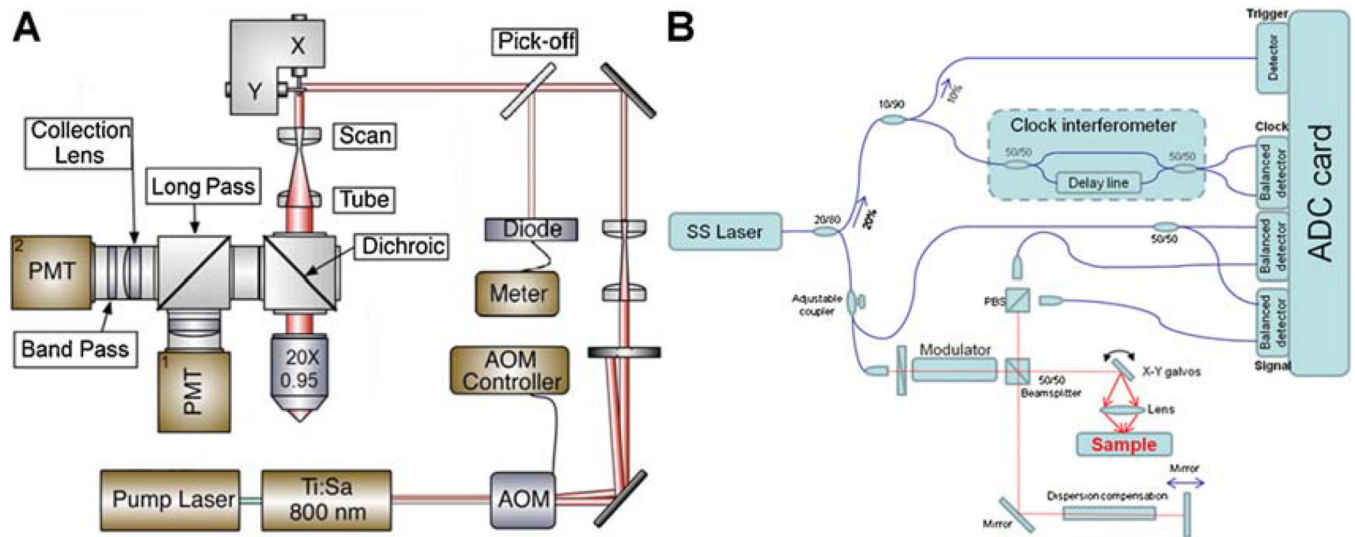
Fig. 3. Schematic diagrams of (A) TPL microscopy and (B) intensity OCT system. PMT, photomultiplier tube; AOM, acousto-optic modulator; SS, swept source.
