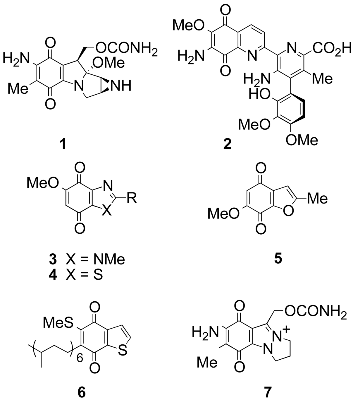
Figure 1. Some heterocyclic quinones.
