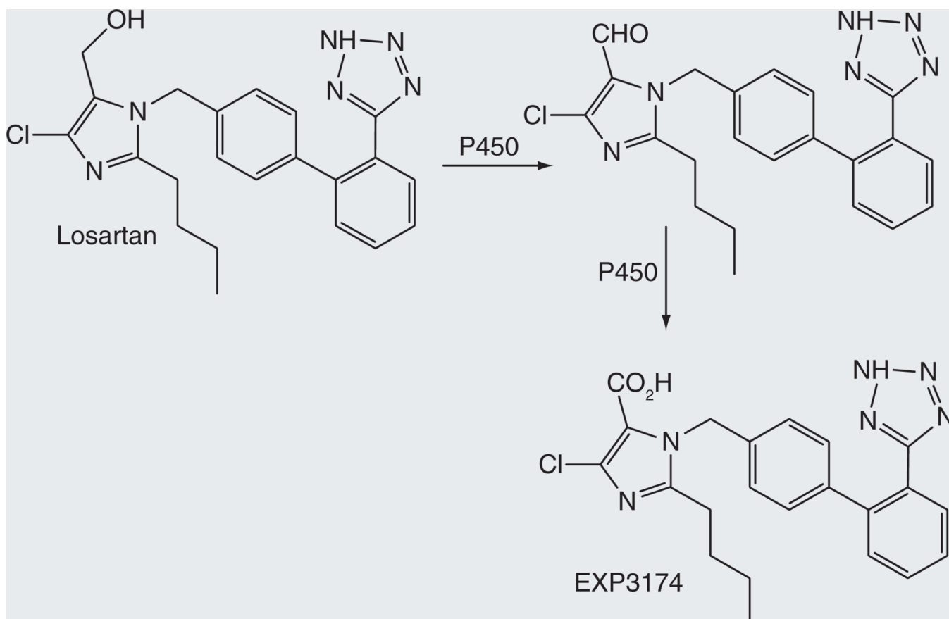
Figure 16. Two-step oxidation of losartan to the biologically active metabolite EXP3174.
