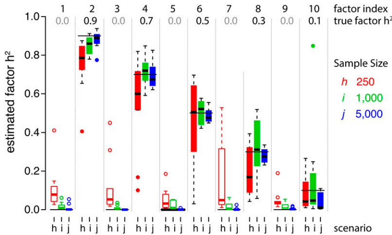
Figure 3 BSFG accurately estimates the heritability of latent traits. Distributions of factor h^2 estimates for scenarios h – j . These scenarios differed in the number of individuals sampled. Ten latent traits with h^2 's between 0.0 and 0.9 were generated in each simulation. After fitting our factor model to each simulated data set, the estimated factors were matched to the true latent traits based on the trait-loading vector angles. Each box plot shows the distribution of h^2 estimates for each simulated factor across 10 simulations. Note that the trait loadings for each factor differed in each simulation; only the h^2 values remained the same. Thin horizontal lines in each column show the simulated h^2 values. Colors correspond to the scenario, and solid boxes/circles are used for factors with h^2 > 0.0 .
