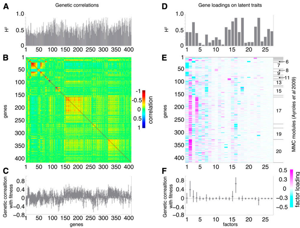
Figure 5 Among-line covariance of gene expression and competitive fitness in Drosophila is modular. (A–C) Genetic (among-line) architecture of 414 gene expression traits measured in adult flies of 40 wild-caught lines (Ayroles et al. 2009). (A) Posterior mean broad-sense heritabilities ( H^2 ) of the 414 genes. (B) Heat map of posterior mean genetic correlations among these genes. (C) Posterior mean estimates and 95% highest posterior density (HPD) intervals for genetic correlations between each gene and competitive fitness. For comparison, see Ayroles et al. (2009, Figure 7a). (D–F) Latent trait structure underlying gene expression covariances. (D) Posterior mean H^2 for each estimated latent trait. (E) Heat map of posterior mean \Lambda matrix showing gene loadings on each latent trait. (F) Posterior mean estimates and 95% HPD intervals for genetic correlations between each latent trait and competitive fitness. The right axis of E groups genes into modules inferred using modulated modularity clustering (Ayroles et al. 2009; Stone and Ayroles 2009).
