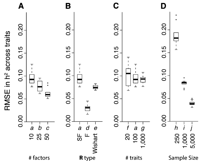
Figure 4 BSFG estimates of individual trait heritability are accurate. The heritability of each individual trait was calculated as h_i^2 = \mathbf{G}_{ii}/\mathbf{P}_{ii} . RSME = \sqrt{(1/p)\sum_{i=1}^p(\hat{h}_i^2 - h_i^2)^2} was calculated for each simulation. Box plots show the distribution of RMSE values for each scenario. (A) Increasing numbers of simulated factors. (B) Different types of \mathbf{R} matrices. (C) Different numbers of traits. (D) Different numbers of sampled individuals.
