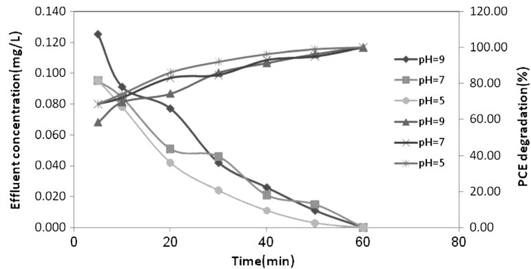
Figure 5 Degradation of aqueous solution of 3 mg/L at different pH subjected to ultrasound and UVC/H 2 O 2 (100 mg/L); T = 25°C.
