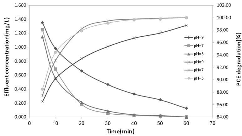
Figure 3 Degradation of aqueous solution of 10 mg/L at different pH subjected to ultrasound and UVC/H 2 O 2 (100 mg/L); T = 25°C.
