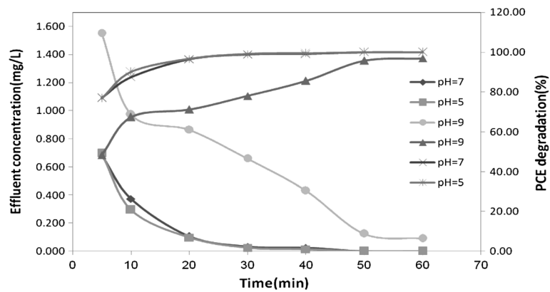
Figure 4 Degradation of aqueous solution of 0.3 mg/L at different pH subjected to ultrasound and UVC/H 2 O 2 (100 mg/L); T = 25°C.
