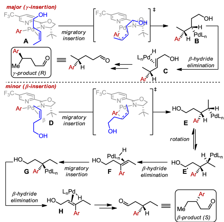
Scheme 1. Mechanistic analysis of stereochemical course.
