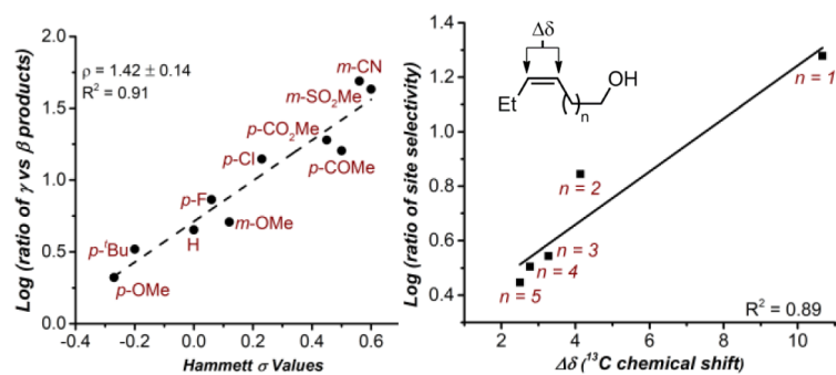
Figure 2. Left: Plot of Log of site-selectivity versus Hammett \sigma -values derived from the scope presented in Table 2. Right: Plot of Log of site-selectivity versus \Delta\delta 13 C chemical shift.
