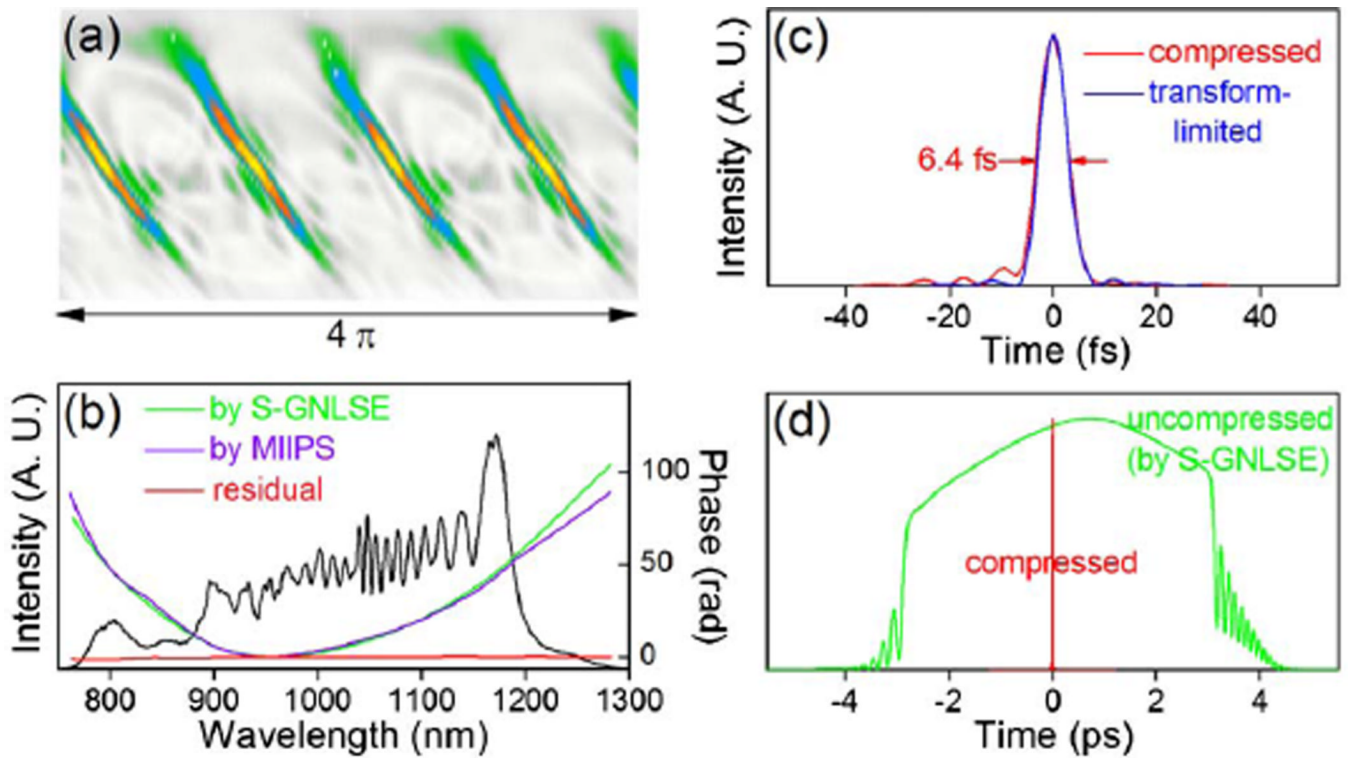
Fig. 2. (Color online) (a) Typical MIIPS trace after pulse measurement and compression; (b) comparison of measured (violet curve) and calculated (green curve) spectral phases, along with residual spectral phase (red curve) and pulse spectrum (black curve); (c) temporal intensity profiles of compressed pulse (red curve) and the corresponding transform-limited pulse (blue curve); (d) temporal intensity profiles of uncompressed (green curve) and compressed (red curve) pulses.
