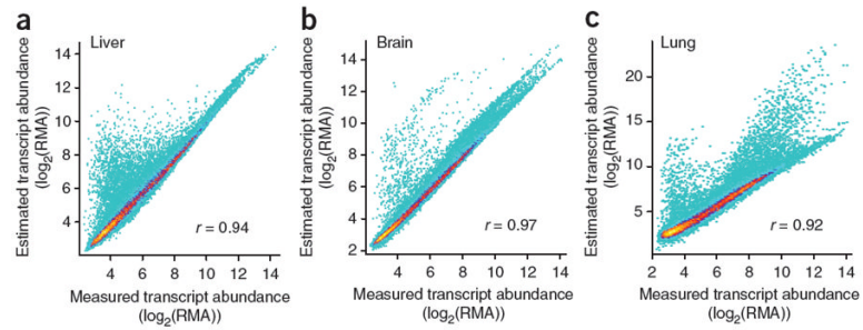
Figure 2. Statistical deconvolution of complex tissues yields accurate estimates of pure tissue-subset expression. (a–c) Density plots of estimated tissue-specific gene expression deconvoluted from mixed tissue samples plotted against measured gene expression from individual tissues. Color represents point density from a single probe (cyan) to 100 probes (yellow). RMA, robust multichip average.
