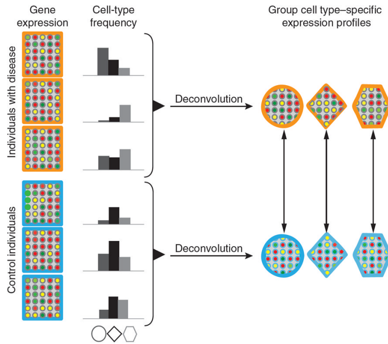
Figure 1. Overview of csSAM. Different cell types are denoted by circles, diamonds and hexagons. csSAM identifies cell type-specific differential expression, as shown by the arrows on the right.
