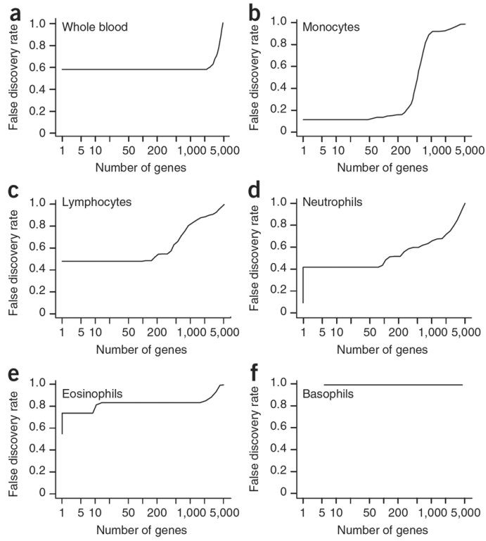
Figure 3. csSAM reveals cell type-specific differential expression undetectable at heterogeneous tissue level. (a–f) Differential expression analysis in whole blood (a) and the indicated cell types (b–f) between samples from individuals with acute rejection and stable post-transplant course.
