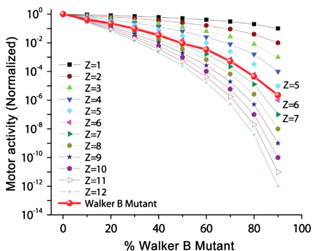
Fig. 5. Viral assembly inhibition assay using a binomial distribution revealing that gp16 is a hexamer in the DNA packaging motor (Trottier and Guo, 1997). Theoretical plot of percent Walker B mutant gp16 versus yield of infectious virions in in vitro phage assembly assays. Predictions were made with the equation (p+q)^Z = \binom{Z}{0}p^Z + \binom{Z}{1}p^{Z-1}q + \binom{Z}{2}p^{Z-2}q^2 + \dots + \binom{Z}{Z-1}pq^{Z-1} + \binom{Z}{Z}q^Z = \sum_{M=0}^Z \binom{Z}{M}p^{Z-M}q^M , where p is the percentage of wild-type eGFP-gp16; q is the percentage of eGFP-gp16/ED; Z , is the total number of eGFP-gp16 per procapsid or gp3-DNA; M is the number of mutant eGFP-gp16 in the phi29 DNA packaging motor; and p+q=1 (Trottier and Guo, 1997).
