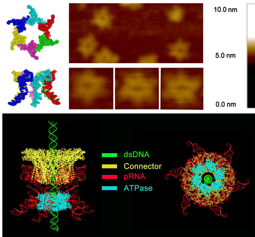
Fig. 1. Depiction of the phi29 DNA packaging motor structure and function. A schematic of hexameric pRNA (left, top) and AFM images of loop-extended hexameric pRNA (top, right) (Shu et al., in press). Illustrations of the phi29 DNA packaging motor and a pRNA hexamer: side view (bottom, left) and bottom view (bottom, right).
