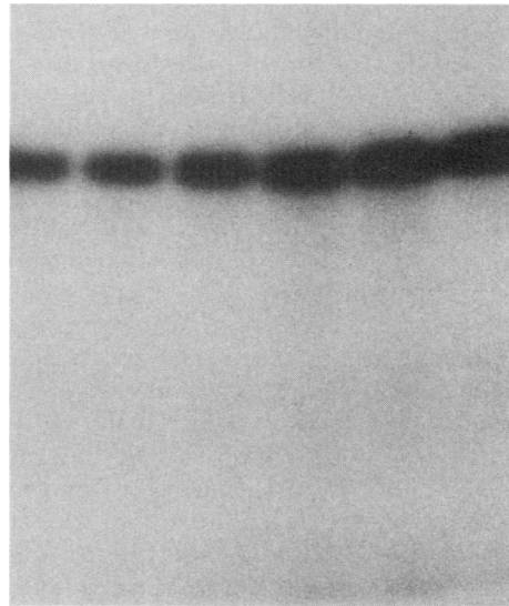
FIGURE 3 SDS polyacrylamide gel electrophoresis and autoradiography of bound Factor VII. Samples (400 \mu\text{l} ) from the ^{125} I-Factor VII reaction mixture described in Fig. 2 were removed at 5, 10, 15, 20, 40, and 60 min (left to right in figure) and centrifuged for 2 min in a microfuge. The cells were resuspended in 50 \mu\text{l} of 0.15 M NaCl, 0.010 M EDTA, 0.05 M Tris, pH 8.1, and 0.02 M benzamidine, and centrifuged once again. A sample of each supernatant was reduced with 5% \beta -mercaptoethanol, and autoradiography performed following SDS polyacrylamide electrophoresis.
