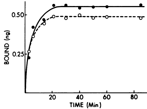
FIGURE 2 Time course of Factors VII and VIIa binding to monocytes. Mixtures containing 4 \times 10^6 /ml monocytes, 6 ng/ml ^{125} I-Factor VII or VIIa and 4 mM \text{CaCl}_2 were incubated at 0°C along with duplicate mixtures to which unlabeled Factor VII or VIIa (2.4 \mu\text{g}/\text{ml} ), respectively, had also been added. Specific binding of Factor VII (●) and Factor VIIa (○) is shown. Nonspecific binding in the Factor VII and VIIa mixtures was 16 and 19%, respectively, of the total maximal binding.
