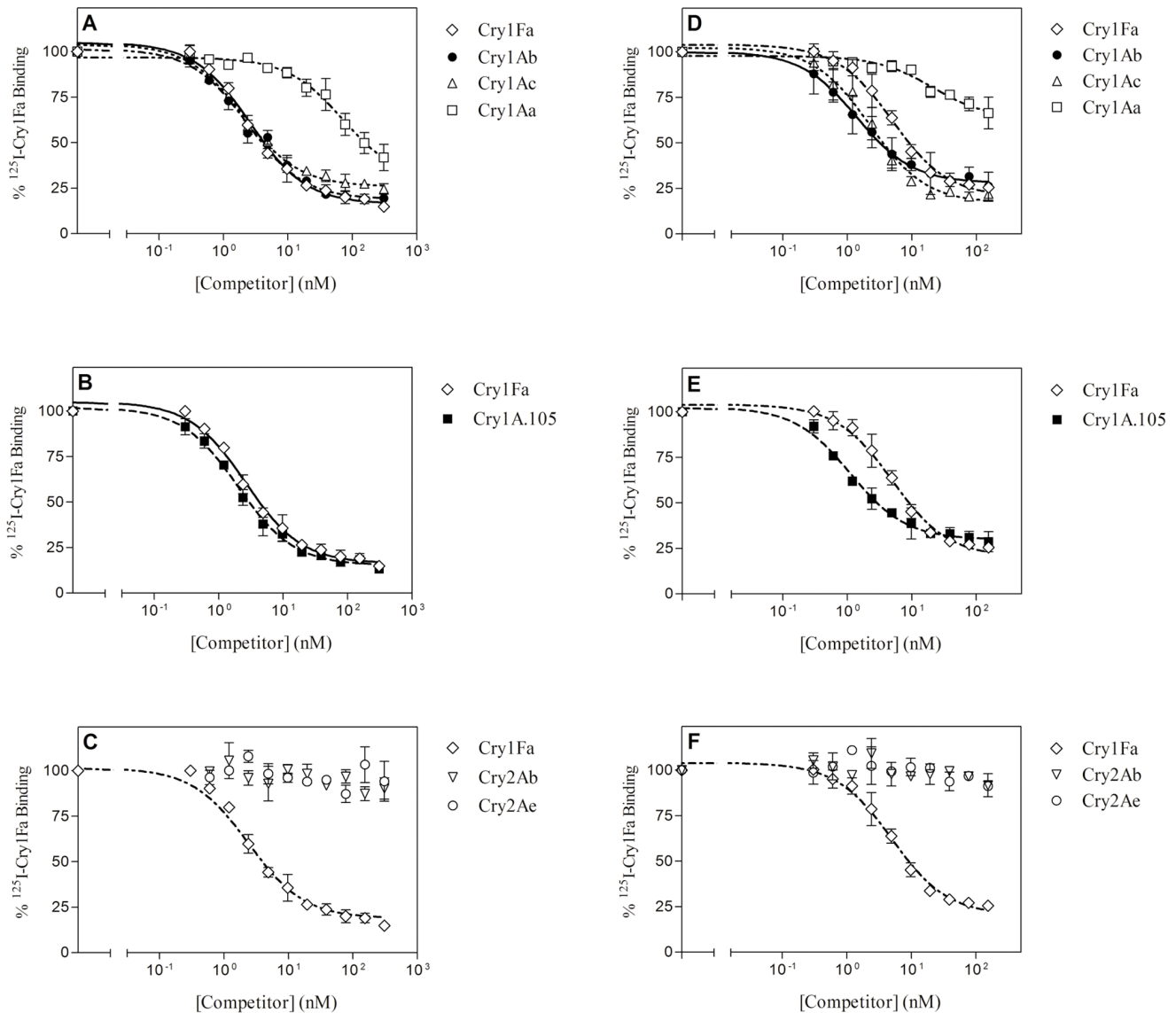
Figure 4. Competition binding experiments with ^{125}\text{I} -Cry1Fa. Curves represent total binding of ^{125}\text{I} -Cry1Fa at increasing concentrations of unlabeled competitor, using BBMV from O. nubilalis (A, B, and C) or from S. frugiperda (D, E, and F). Each competition experiment (data points in duplicate) was replicated two to three times in O. nubilalis (competition with Cry1Ab and Cry1Ac in O. nubilalis was replicated three times) and two times in S. frugiperda and the error bars represent the standard error of the mean. doi:10.1371/journal.pone.0068164.g004
