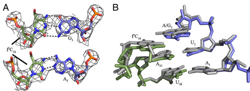
Fig. 3. Geometry of the wobble base pair and codon•anticodon interaction. (A) The electron density shows that both the f 5 C 34 •G 3 and f 5 C 34 •A 3 base pairs are in Watson–Crick geometry. ASL carbons are colored green, and mRNA carbons are blue (m2F O -dF C contoured at 1.5 \sigma ). (B) Superposition of the hmASL Met f5CAU •AUG complex with the hmASL Met f5CAU •AUA structure aligned with respect to the mRNA residues. The overlay reveals a nearly identical orientation of the codon•anticodon interaction between the AUA-bound and AUG-bound structures. The ASL and mRNA residues for the AUA-bound structures are green and blue, respectively. The ASL and mRNA residues of the AUG-bound structure are both gray.
