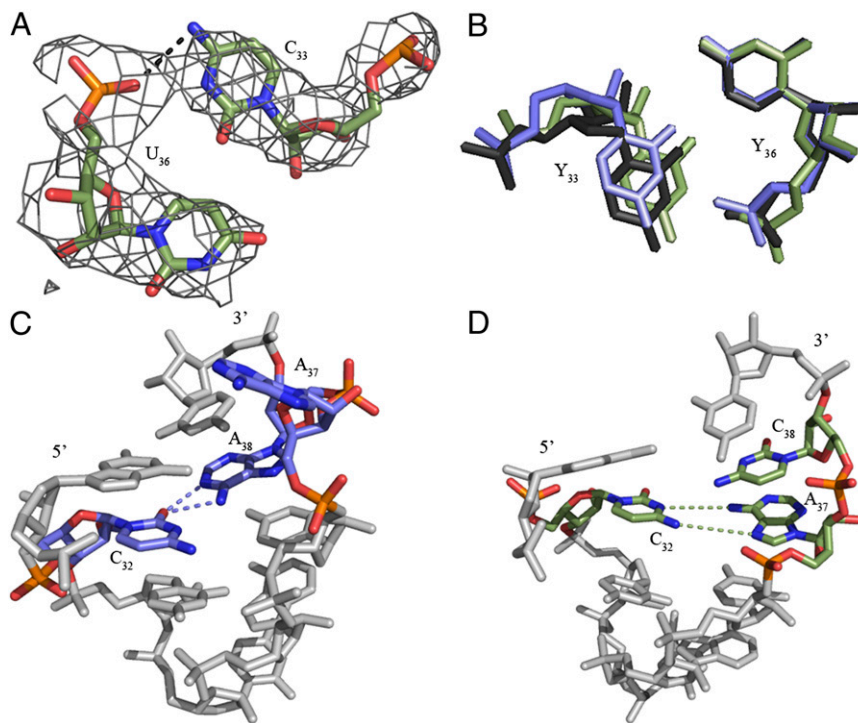
Fig. 2. Unusual features of the hmASL Met f5CAU structure. (A) A hydrogen bond is able to form between C 33 N4 and the phosphate of U 36 . ASL carbons are colored green, and mRNA carbons are blue (m2F O -dF C contoured at 1.5 \sigma ). (B) hmASL Met f5CAU (green) is superimposed with E. coli elongator tRNA Lys UUU (blue) and human elongator tRNA Lys UUU (black), showing a slightly distorted conformation. (C) In E. coli tRNA Met CAU , the cross-loop interaction involves the familiar C 32 •A 38 non-canonical base pair with A 37 displaced from the loop, where it cannot participate in base stacking. (D) A cross-loop interaction in hmASL Met f5CAU involves a unique interaction between C 32 and A 37 that consists of a base pair between the Watson–Crick edge of C 32 and the Hoogsteen edge of A 37 .
