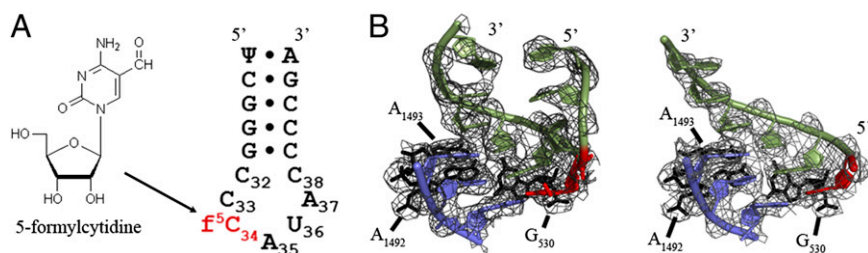
Fig. 1. hmASL Met f5CAU secondary structure and A-site codon•anticodon interaction. (A) The ASL was synthesized as a heptadecamer containing two modifications: pseudouridine at position 27 and 5-fomylcytidine at position 34. (B) The structure of hmASL Met f5CAU bound to AUG (Left) showed strong electron density for ASL residues 31–39, whereas when bound to AUA (Right), electron density was strong for only residues 34–39. In both structures, the ASL is in green, the mRNA codon is in blue, and the A-site interacting residues (G 530 , A 1492 , and A 1493 ) are in black (2mF O -dF C contoured at 1.5 \sigma ). The f 5 C 34 modification is colored red.
