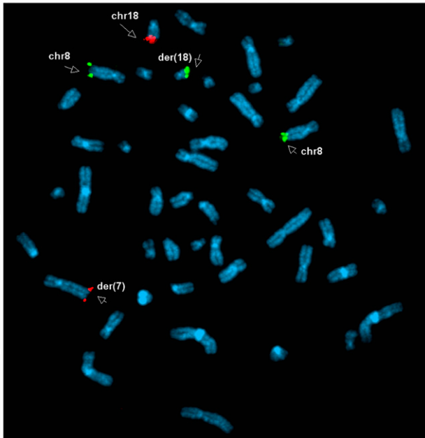
A FISH analysis of GM00657: Green: D8S1925; Red: D18S1380
