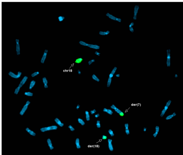
B FISH analysis of GM00657: Green: wcp18
