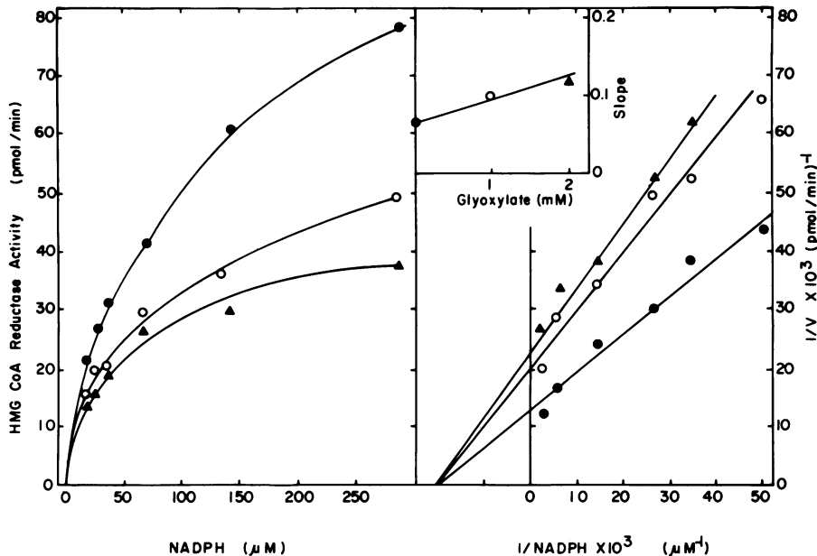
FIGURE 3 Noncompetitive inhibition of HMG CoA reductase by glyoxylate, with respect to NADPH. Microsomal reductase (100 \mu l, 4.5 mg protein) was mixed with either 800 \mu l buffer D containing 70 mM KCl or 288 \mu l of 10 mM glyoxylate plus 512 \mu l buffer containing 70 mM KCl and incubated for 20 min at 37°C. 45- \mu l portions of this mixture were then combined in a final volume of 70 \mu l of buffer D containing 70 mM KCl, with 15 \mu l of reductase substrate-cofactor solution and NADPH at the indicated final concentrations. Reductase activity was measured in a 15-min incubation at 37°C. Concentrations of glyoxylate present during reductase were 0 mM (●), 1 mM (○), 2 mM (▲). Data are for duplicate analyses. (Left) Reductase activity as a function of NADPH concentration. (Right) Reciprocal velocity as a function of reciprocal NADPH concentration. (Insert) Secondary plot of the slope as a function of glyoxylate concentration. The K_m of reductase for NADPH was 51 \mu M. The K_i for glyoxylate with respect to NADPH was 2.7 mM.
