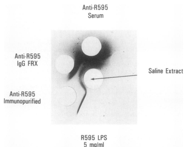
FIGURE 3 Immunodiffusion analysis of the anti-R595 LPS antiserum using a sonicated saline/EDTA extract of whole S. minnesota R595 bacteria and purified R595 LPS as antigen. See the text for experimental details.
