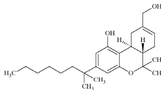
Fig. (45). Chemical structure of dexanabinol.
