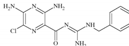
Fig. (52). Chemical structure of benzamil.
