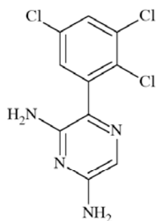
Fig. (11). Chemical structure of JZP-4.
