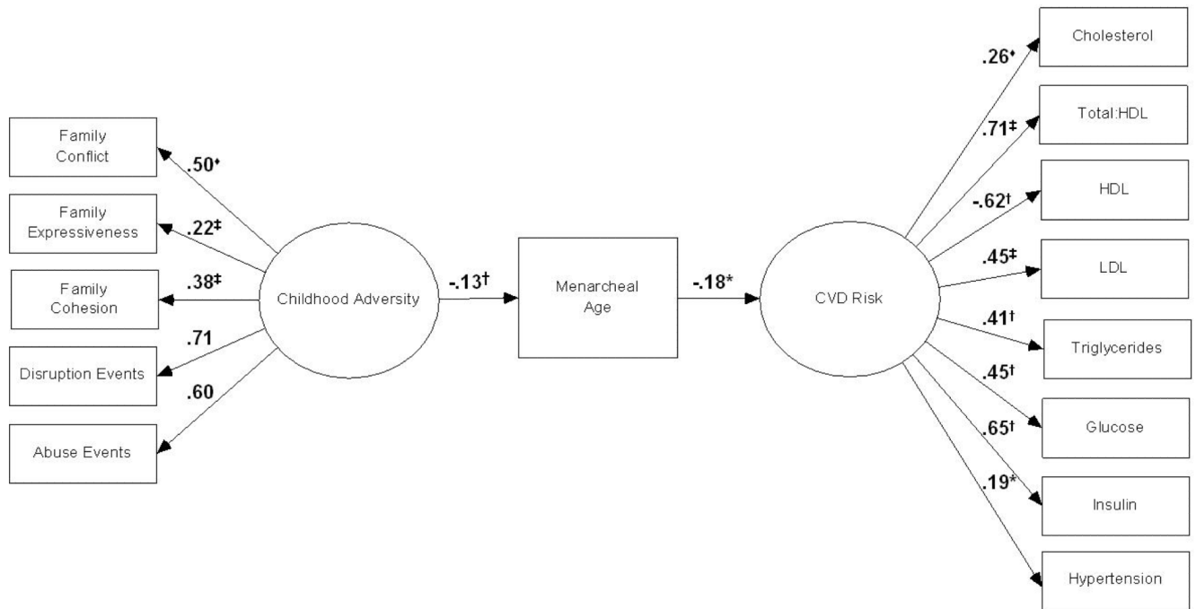
Figure 1. Covariate-adjusted model depicting SEM standardized estimates of associations between childhood adversity, menarcheal age, and CVD risk.
