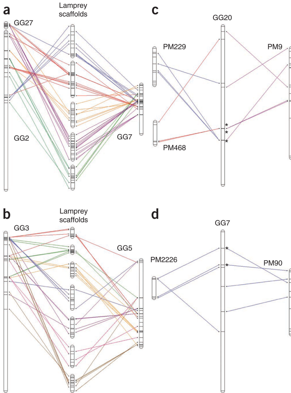
Figure 3. Conserved synteny and duplication in the lamprey and gnathostome (chicken) genomes. (a–d) The locations of presumptive lamprey-chicken orthologs (including duplicates) are plotted relative to their physical positions on chromosomes and scaffolds and are connected by colored lines. (a,b) Pairs of chicken chromosomes that correspond to a series of lamprey scaffolds. (a) Ten lamprey loci are present as duplicate copies in the chicken genome, and 59 are present as single copies. (b) Twelve lamprey loci are present as duplicate copies in the chicken genome, and 54 are present as single copies. (c,d) Pairs of lamprey scaffolds that correspond to individual chicken chromosomes. (c) Three chicken loci are present as duplicate copies on syntenic lamprey scaffolds. (d) Two chicken loci are present as duplicate copies on syntenic lamprey scaffolds. Asterisks indicate duplicates.
