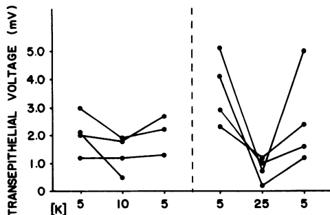
FIGURE 3 Effect of increasing K concentration (in millimolars) in bath and lumen on transepithelial voltage across MTALH of the rabbit. Time course was similar to the experiments conducted on mouse MTALH (Figs. 1 and 2). Solution 1 was used (328 mosmol/kg \text{H}_2\text{O} ) and K replaced Na.
