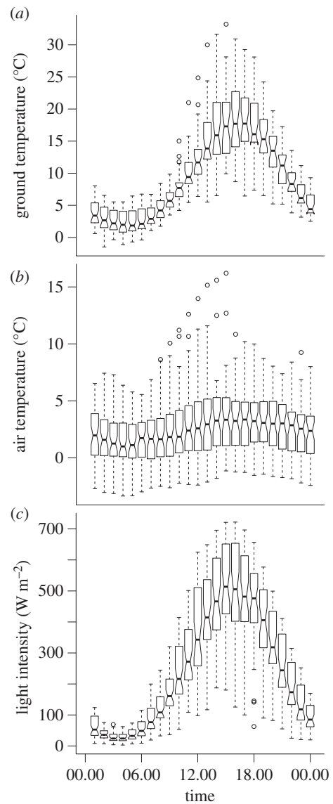
Figure 1. Daily environmental cycles in Barrow, Alaska. (a) Ground temperature ( ^{\circ} C). (b) Air temperature ( ^{\circ} C). (c) Light intensity ( \text{W m}^{-2} ). Shown are box plots with hourly median, 25th and 75th percentile, 9th and 91st percentile, and outliers. Ground temperature data were recorded between 14 June and 18 July 2006 near 27 nests of pectoral sandpipers using iButtons (accuracy \pm 1^{\circ} C). Air temperature (2 m above ground) and light intensity data were collected by weather stations located in Barrow from 1 June to 20 July 2008. These data were kindly provided by the NOAA Earth System Research Laboratory ( http://www.esrl.noaa.gov ). Note that light intensity was measured with an unshaded pyranometer (results referred to as 'global'), and may yield erroneous results at extremes of zenith angle (R. Stone 2012, personal communication). Near-zero values can occur at low solar elevation in cloudy conditions.
