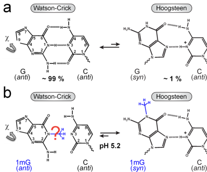
Figure 1. Schematic of the equilibrium between a G•C WC and HG base pair. (a) The transition from a ground state WC to a transient state HG base pair, with relative populations measured by NMR relaxation dispersion, 3 requires an anti -to- syn rotation around the glycosidic bond ( \chi ) and creates a stabilizing H-bond upon C N3 protonation. (b) Methylation at G N1 favors formation of a ground state HG base pair at pH 5.2. 3
