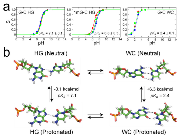
Figure 3. Constant pH MD simulations of WC and HG base pair protonation. (a) Titration curves obtained from 3 independent runs of single-site CPHMD MS \lambda D simulations of a G•C HG base pair, its 1mG analog, and a G•C WC base pair. (b) Corresponding structures for the neutral and protonated WC and HG base pairs and predicted free energy differences at pH 7, depicted in the context of the proposed 4-state equilibrium.
